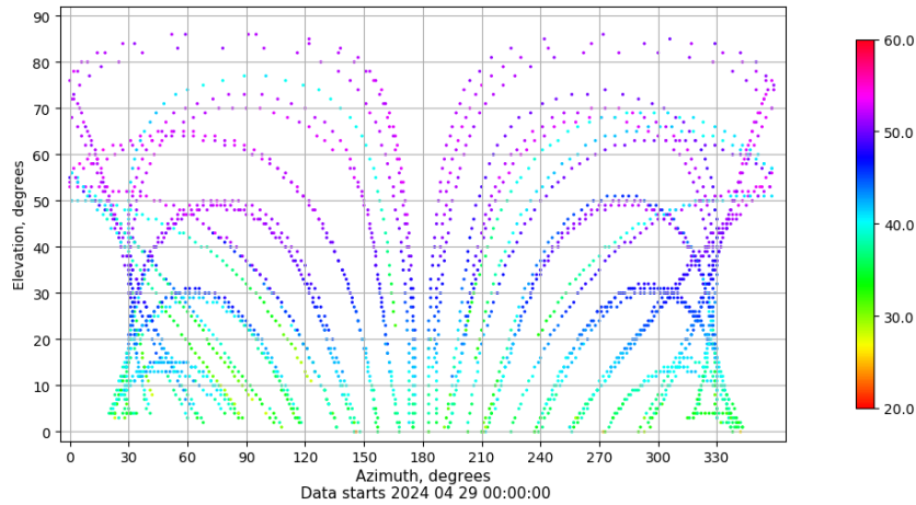
Azimuth-elevation plot for station TAR2. Signal to Noise S1C Data file TAR200ESP_R_2024120.xtr
