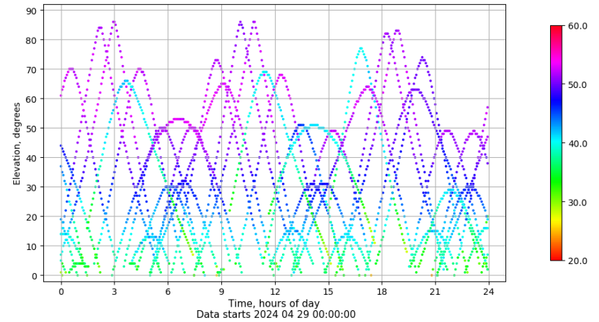
Time-elevation plot for station TAR2. Signal to Noise S1C Data file TAR200ESP_R_2024120.xtr
