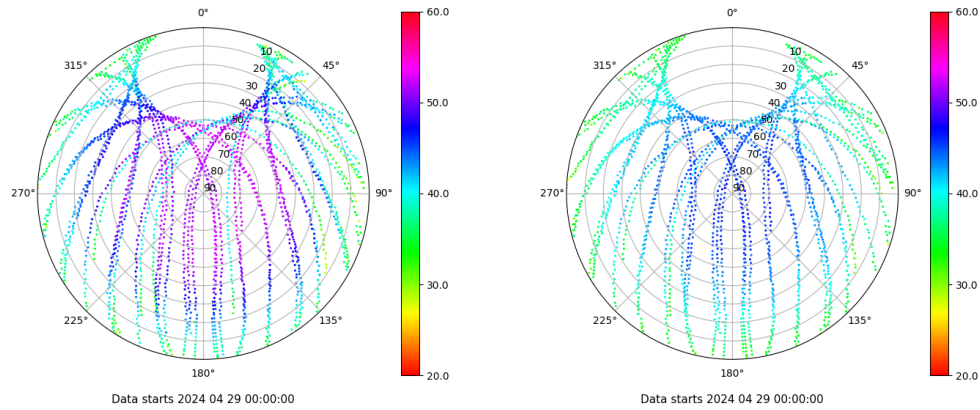
Skyplot for station TAR2. Signal to Noise S1C Data file TAR200ESP_R_2024120.xtr Skyplot for station TAR2. Signal to Noise S2C Data file TAR200ESP_R_2024120.xtr
