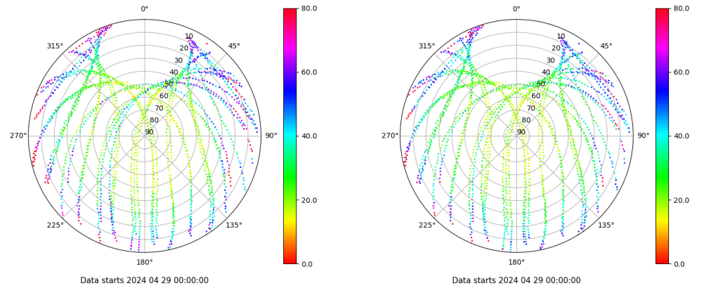
Skyplot for station TAR2. Parameter M1C Data file TAR200ESP_R_2024120.xtr Skyplot for station TAR2. Parameter M2C Data file TAR200ESP_R_2024120.xtr
