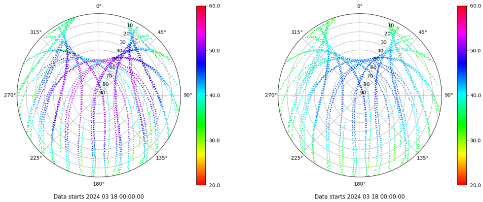
Skyplot for station TAR2. Signal to Noise S1C Data file TAR200ESP_R_2024078.xtr Skyplot for station TAR2. Signal to Noise S2C Data file TAR200ESP_R_2024078.xtr
