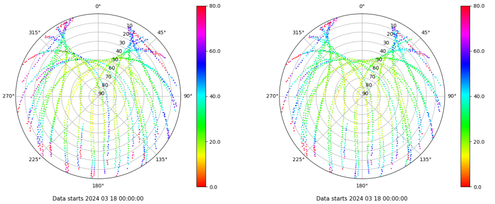
Skyplot for station TAR2. Parameter M1C Data file TAR200ESP_R_2024078.xtr Skyplot for station TAR2. Parameter M2C Data file TAR200ESP_R_2024078.xtr
