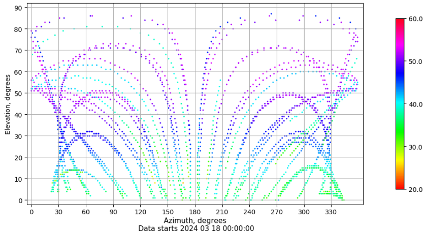
Azimuth-elevation plot for station TAR2. Signal to Noise S1C Data file TAR200ESP_R_2024078.xtr
