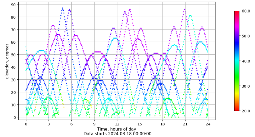
Time-elevation plot for station TAR2. Signal to Noise S1C Data file TAR200ESP_R_2024078.xtr
