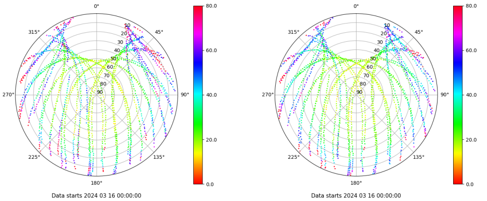
Skyplot for station TAR2. Parameter M1C Data file TAR200ESP_R_2024076.xtr Skyplot for station TAR2. Parameter M2C Data file TAR200ESP_R_2024076.xtr
