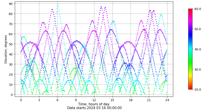
Time-elevation plot for station TAR2. Signal to Noise S1C Data file TAR200ESP_R_2024076.xtr
