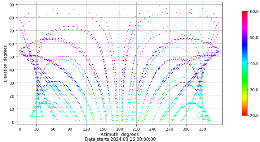
Azimuth-elevation plot for station TAR2. Signal to Noise S1C Data file TAR200ESP_R_2024076.xtr
