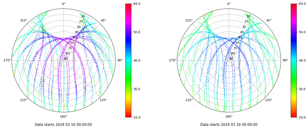
Skyplot for station TAR2. Signal to Noise S1C Data file TAR200ESP_R_2024076.xtr Skyplot for station TAR2. Signal to Noise S2C Data file TAR200ESP_R_2024076.xtr
