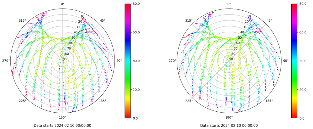
Skyplot for station TAR2. Parameter M1C Data file TAR200ESP_R_2024041.xtr Skyplot for station TAR2. Parameter M2C Data file TAR200ESP_R_2024041.xtr
