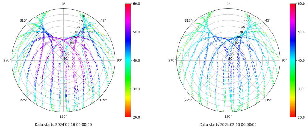
Skyplot for station TAR2. Signal to Noise S1C Data file TAR200ESP_R_2024041.xtr Skyplot for station TAR2. Signal to Noise S2C Data file TAR200ESP_R_2024041.xtr
