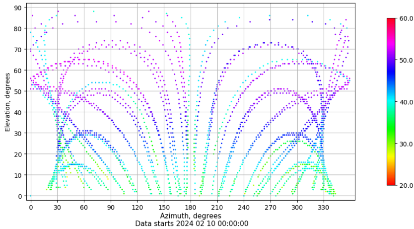
Azimuth-elevation plot for station TAR2. Signal to Noise S1C Data file TAR200ESP_R_2024041.xtr
