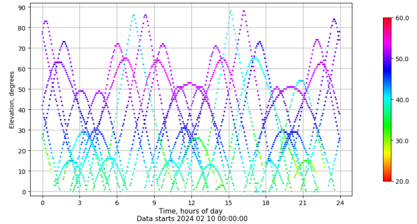
Time-elevation plot for station TAR2. Signal to Noise S1C Data file TAR200ESP_R_2024041.xtr
