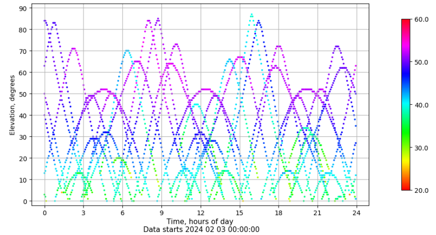
Time-elevation plot for station TAR2. Signal to Noise S1C Data file TAR200ESP_R_2024034.xtr
