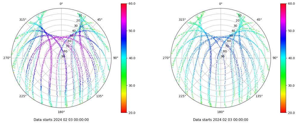
Skyplot for station TAR2. Signal to Noise S1C Data file TAR200ESP_R_2024034.xtr Skyplot for station TAR2. Signal to Noise S2C Data file TAR200ESP_R_2024034.xtr
