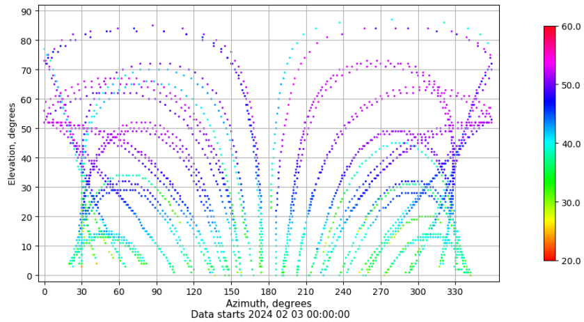
Azimuth-elevation plot for station TAR2. Signal to Noise S1C Data file TAR200ESP_R_2024034.xtr
