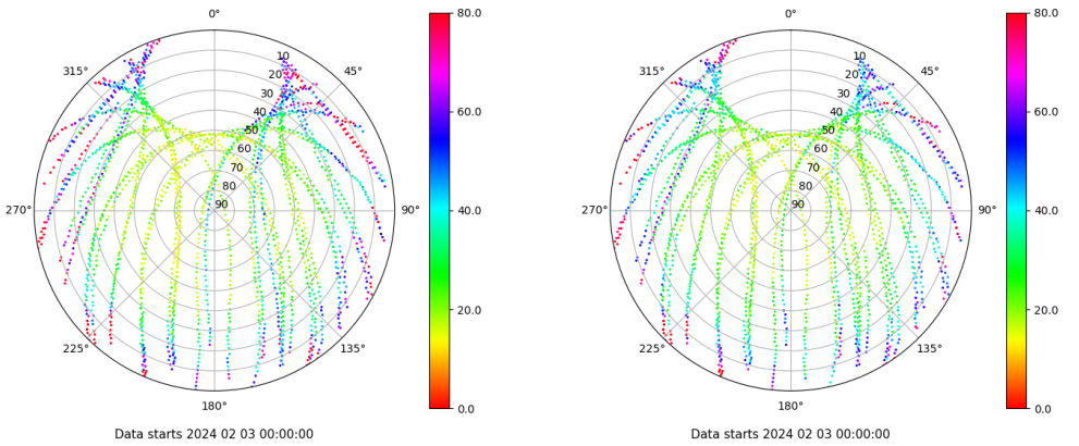
Skyplot for station TAR2. Parameter M1C Data file TAR200ESP_R_2024034.xtr Skyplot for station TAR2. Parameter M2C Data file TAR200ESP_R_2024034.xtr
