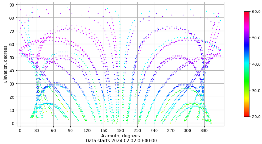
Azimuth-elevation plot for station TAR2. Signal to Noise S1C Data file TAR200ESP_R_2024033.xtr
