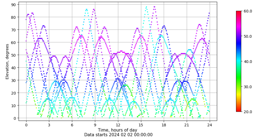
Time-elevation plot for station TAR2. Signal to Noise S1C Data file TAR200ESP_R_2024033.xtr
