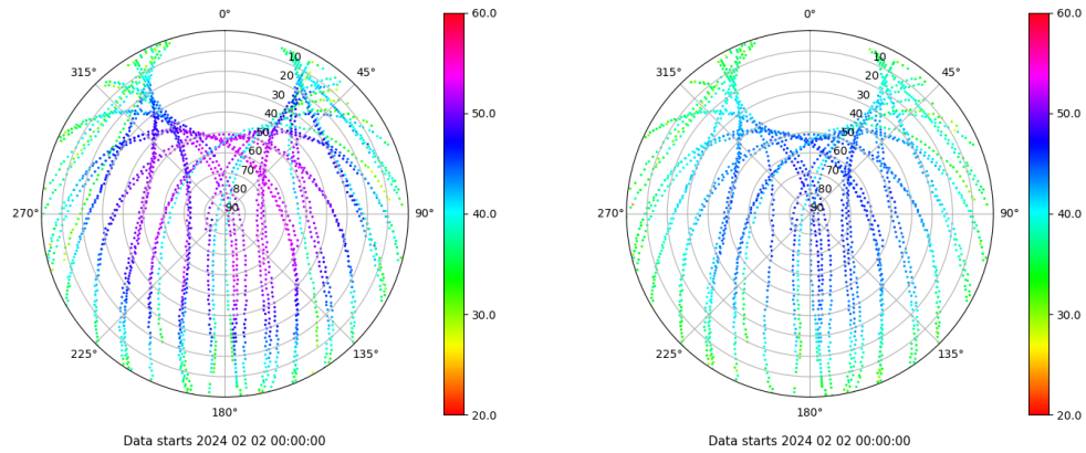
Skyplot for station TAR2. Signal to Noise S1C Data file TAR200ESP_R_2024033.xtr Skyplot for station TAR2. Signal to Noise S2C Data file TAR200ESP_R_2024033.xtr
