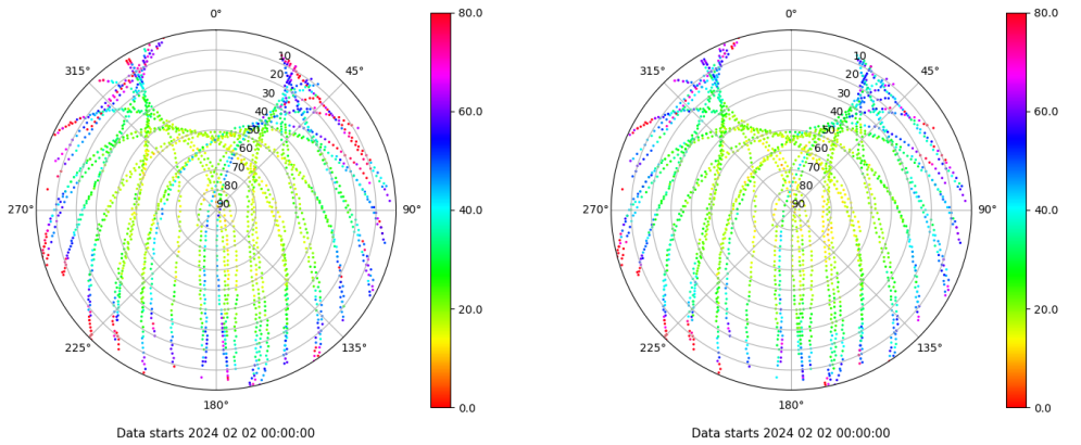
Skyplot for station TAR2. Parameter M1C Data file TAR200ESP_R_2024033.xtr Skyplot for station TAR2. Parameter M2C Data file TAR200ESP_R_2024033.xtr
