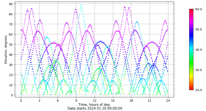
Time-elevation plot for station TAR2. Signal to Noise S1C Data file TAR200ESP_R_2024020.xtr
