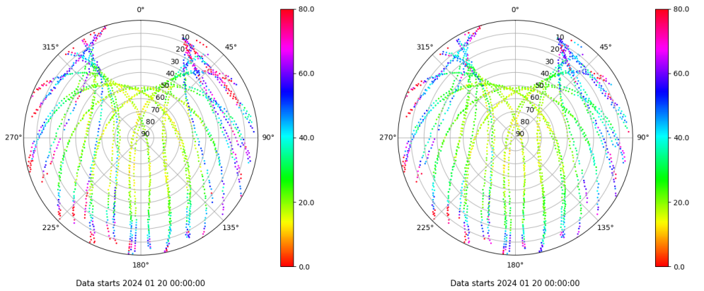
Skyplot for station TAR2. Parameter M1C Data file TAR200ESP_R_2024020.xtr Skyplot for station TAR2. Parameter M2C Data file TAR200ESP_R_2024020.xtr
