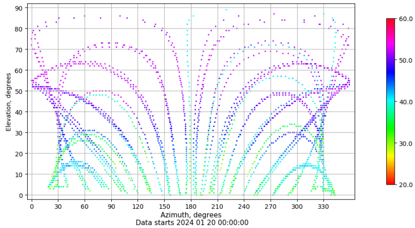
Azimuth-elevation plot for station TAR2. Signal to Noise S1C Data file TAR200ESP_R_2024020.xtr
