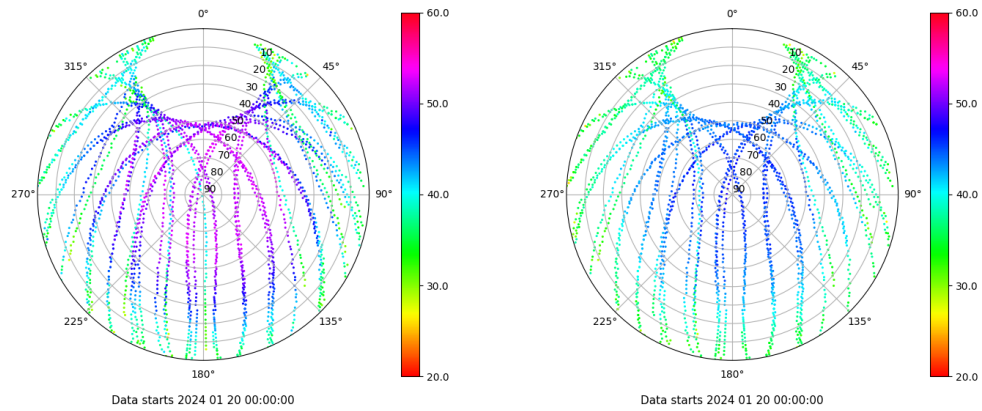
Skyplot for station TAR2. Signal to Noise S1C Data file TAR200ESP_R_2024020.xtr Skyplot for station TAR2. Signal to Noise S2C Data file TAR200ESP_R_2024020.xtr
