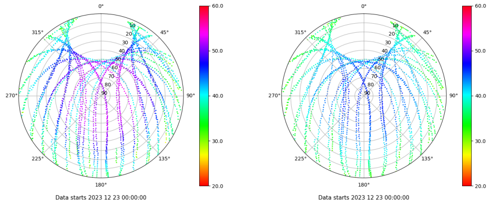
Skyplot for station TAR2. Signal to Noise S1C Data file TAR200ESP_R_2023357.xtr Skyplot for station TAR2. Signal to Noise S2C Data file TAR200ESP_R_2023357.xtr
