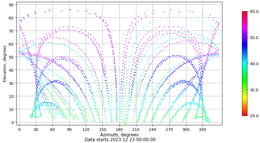
Azimuth-elevation plot for station TAR2. Signal to Noise S1C Data file TAR200ESP_R_2023357.xtr
