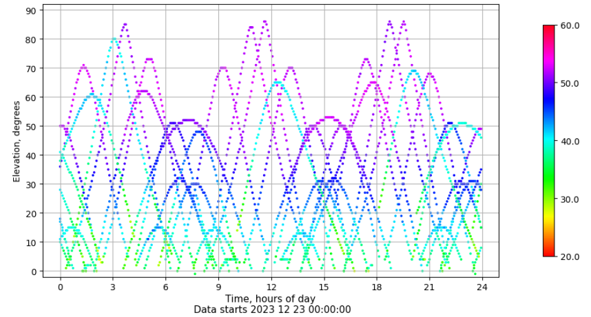
Time-elevation plot for station TAR2. Signal to Noise S1C Data file TAR200ESP_R_2023357.xtr
