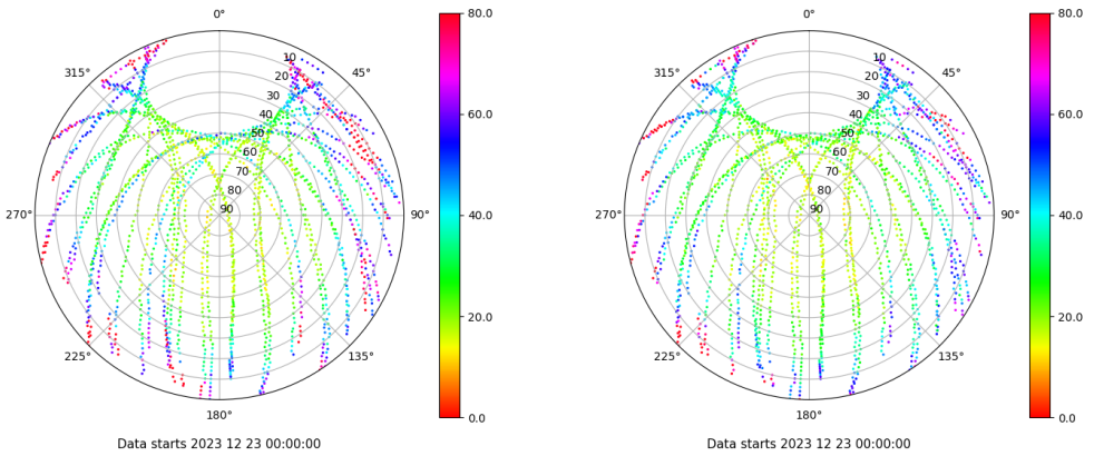
Skyplot for station TAR2. Parameter M1C Data file TAR200ESP_R_2023357.xtr Skyplot for station TAR2. Parameter M2C Data file TAR200ESP_R_2023357.xtr
