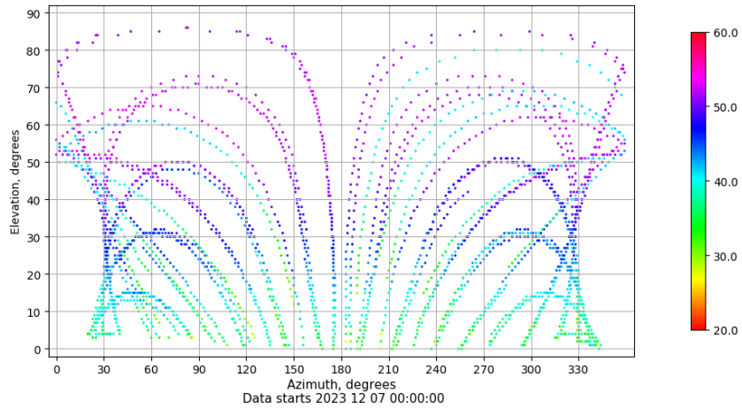
Azimuth-elevation plot for station TAR2. Signal to Noise S1C Data file TAR200ESP_R_2023341.xtr
