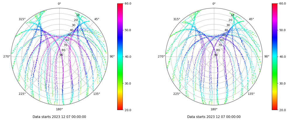
Skyplot for station TAR2. Signal to Noise S1C Data file TAR200ESP_R_2023341.xtr Skyplot for station TAR2. Signal to Noise S2C Data file TAR200ESP_R_2023341.xtr
