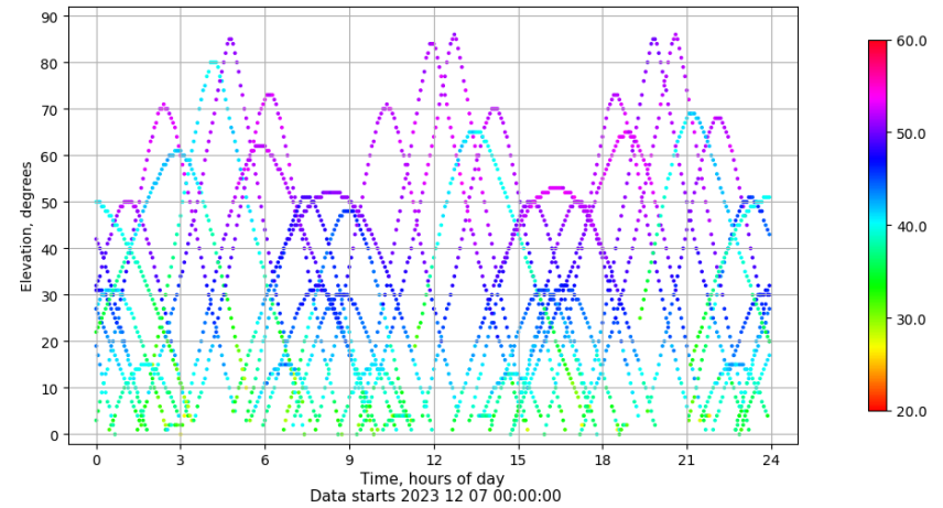
Time-elevation plot for station TAR2. Signal to Noise S1C Data file TAR200ESP_R_2023341.xtr
