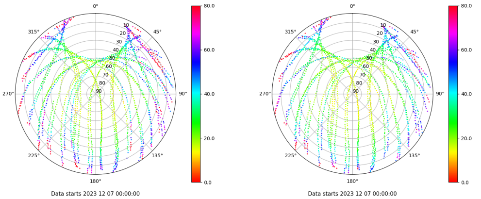
Skyplot for station TAR2. Parameter M1C Data file TAR200ESP_R_2023341.xtr Skyplot for station TAR2. Parameter M2C Data file TAR200ESP_R_2023341.xtr
