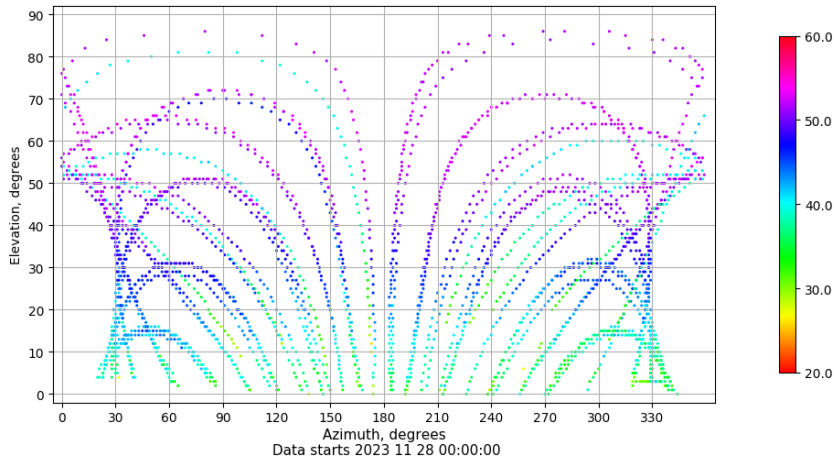
Azimuth-elevation plot for station TAR2. Signal to Noise S1C Data file TAR200ESP_R_2023332.xtr
