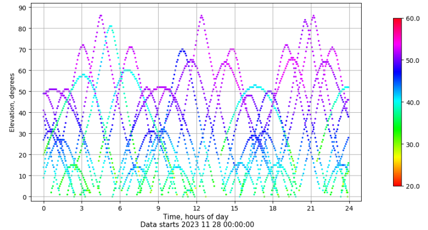
Time-elevation plot for station TAR2. Signal to Noise S1C Data file TAR200ESP_R_2023332.xtr
