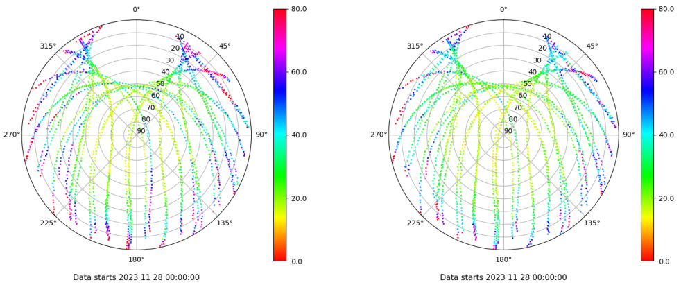
Skyplot for station TAR2. Parameter M1C Data file TAR200ESP_R_2023332.xtr Skyplot for station TAR2. Parameter M2C Data file TAR200ESP_R_2023332.xtr
