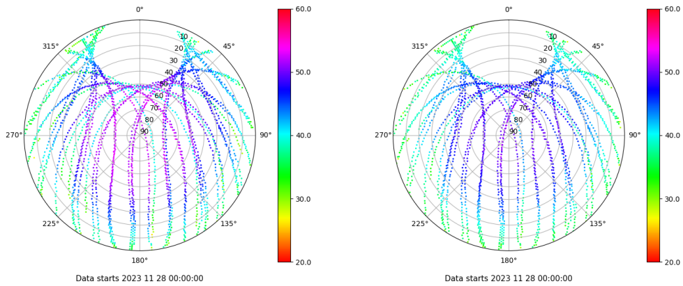
Skyplot for station TAR2. Signal to Noise S1C Data file TAR200ESP_R_2023332.xtr Skyplot for station TAR2. Signal to Noise S2C Data file TAR200ESP_R_2023332.xtr
