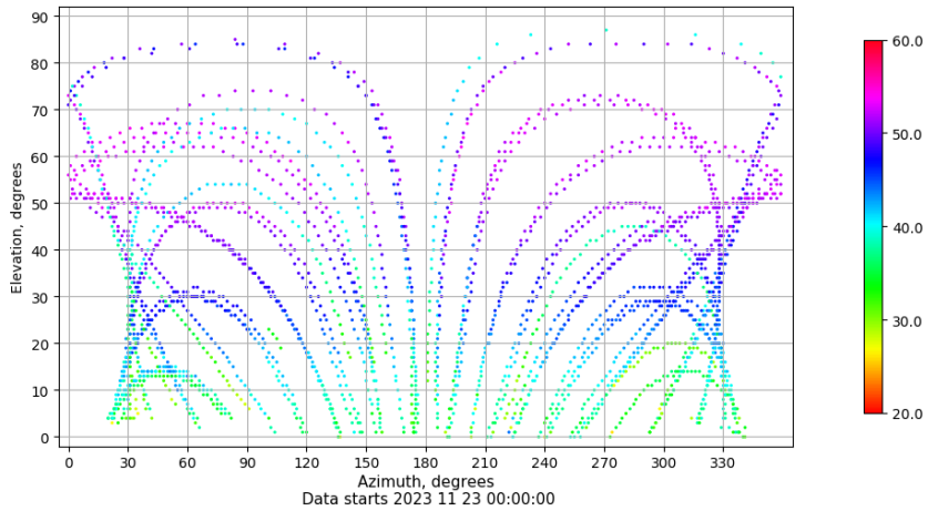
Azimuth-elevation plot for station TAR2. Signal to Noise S1C Data file TAR200ESP_R_2023327.xtr
