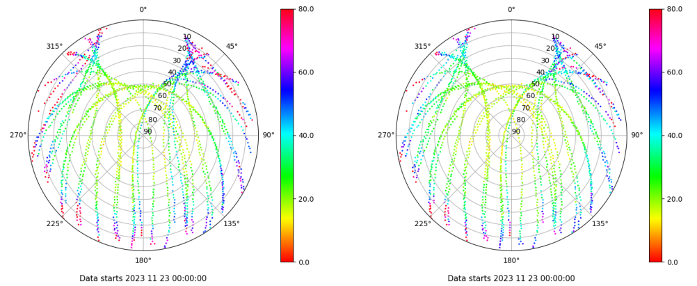
Skyplot for station TAR2. Parameter M1C Data file TAR200ESP_R_2023327.xtr Skyplot for station TAR2. Parameter M2C Data file TAR200ESP_R_2023327.xtr
