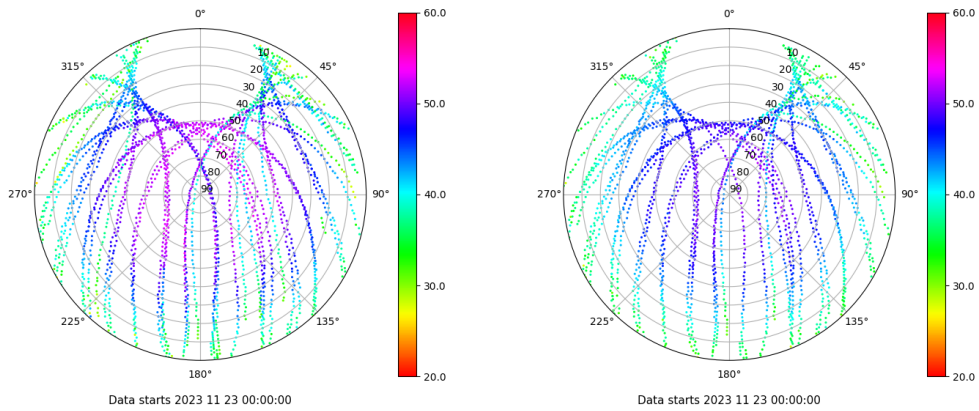
Skyplot for station TAR2. Signal to Noise S1C Data file TAR200ESP_R_2023327.xtr Skyplot for station TAR2. Signal to Noise S2C Data file TAR200ESP_R_2023327.xtr
