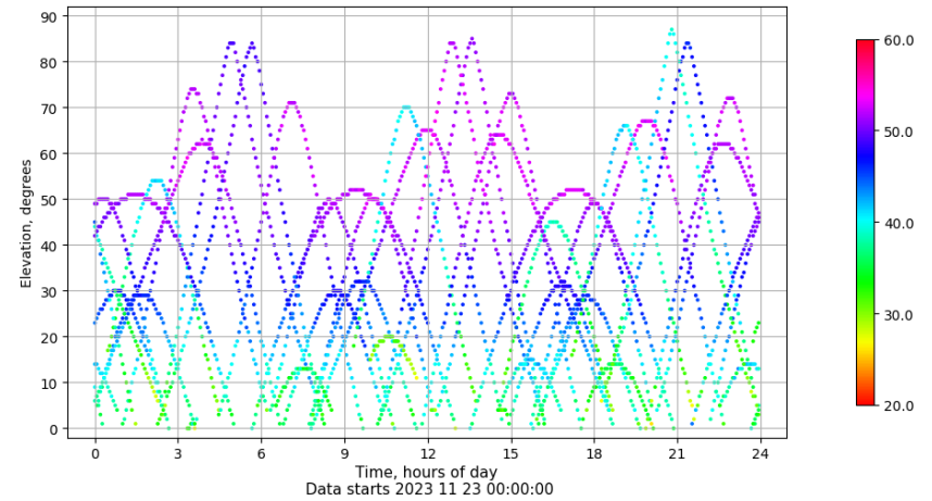
Time-elevation plot for station TAR2. Signal to Noise S1C Data file TAR200ESP_R_2023327.xtr
