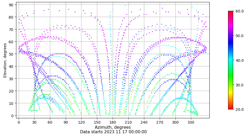
Azimuth-elevation plot for station TAR2. Signal to Noise S1C Data file TAR200ESP_R_2023321.xtr
