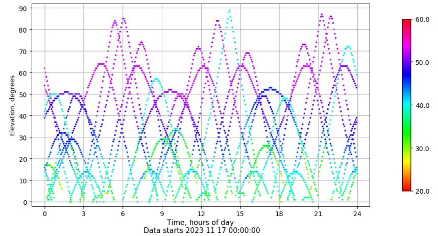
Time-elevation plot for station TAR2. Signal to Noise S1C Data file TAR200ESP_R_2023321.xtr
