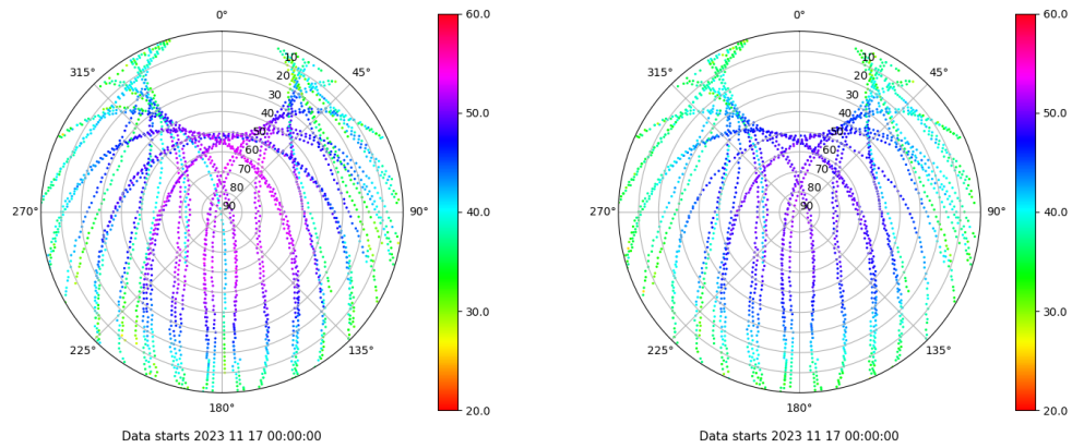
Skyplot for station TAR2. Signal to Noise S1C Data file TAR200ESP_R_2023321.xtr Skyplot for station TAR2. Signal to Noise S2C Data file TAR200ESP_R_2023321.xtr
