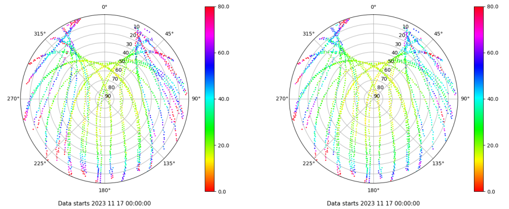
Skyplot for station TAR2. Parameter M1C Data file TAR200ESP_R_2023321.xtr Skyplot for station TAR2. Parameter M2C Data file TAR200ESP_R_2023321.xtr
