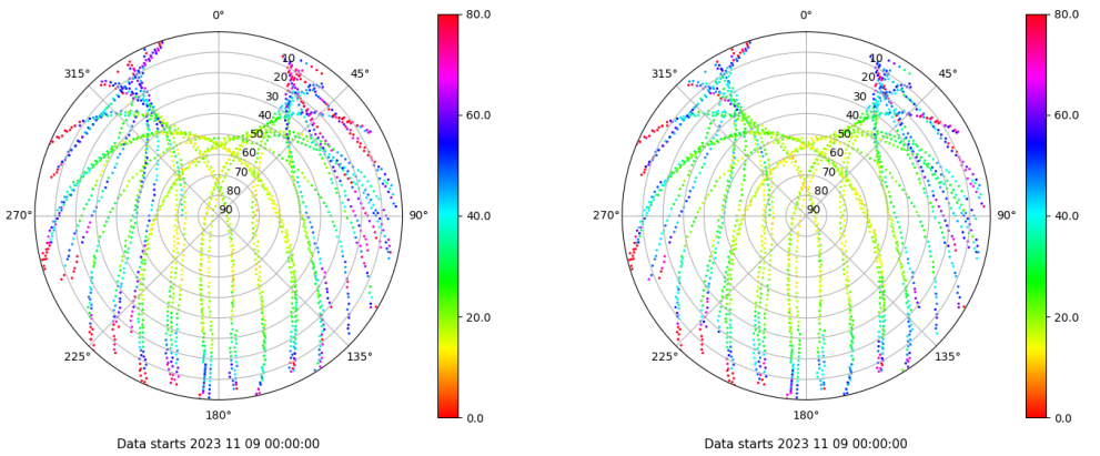
Skyplot for station TAR2. Parameter M1C Data file TAR200ESP_R_2023313.xtr Skyplot for station TAR2. Parameter M2C Data file TAR200ESP_R_2023313.xtr
