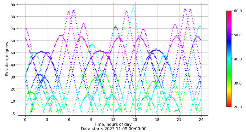
Time-elevation plot for station TAR2. Signal to Noise S1C Data file TAR200ESP_R_2023313.xtr
