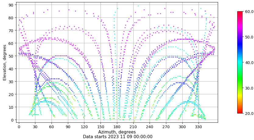
Azimuth-elevation plot for station TAR2. Signal to Noise S1C Data file TAR200ESP_R_2023313.xtr
