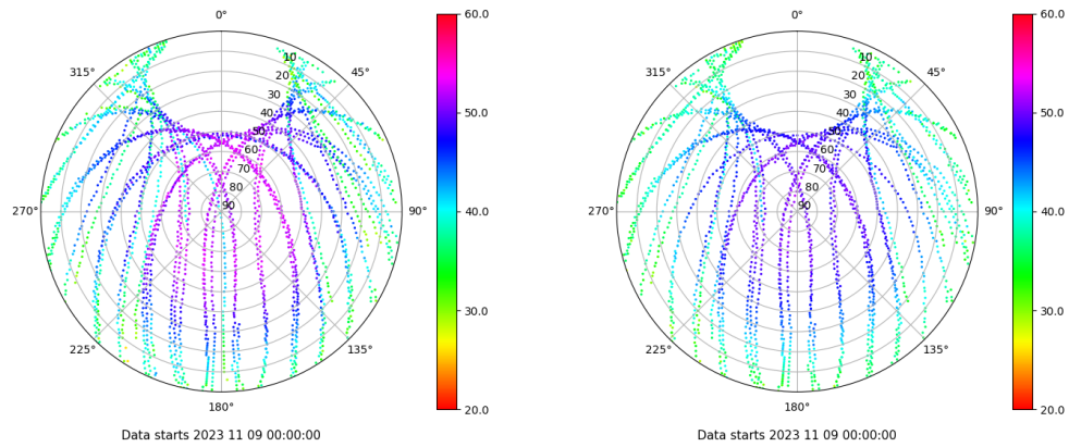
Skyplot for station TAR2. Signal to Noise S1C Data file TAR200ESP_R_2023313.xtr Skyplot for station TAR2. Signal to Noise S2C Data file TAR200ESP_R_2023313.xtr
