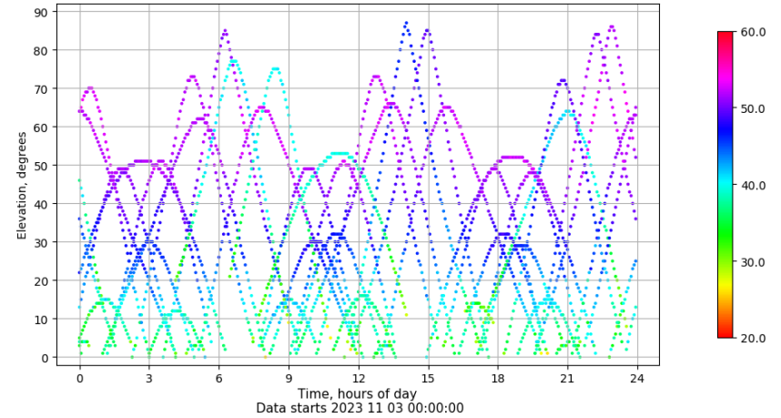
Time-elevation plot for station TAR2. Signal to Noise S1C Data file TAR200ESP_R_2023307.xtr
