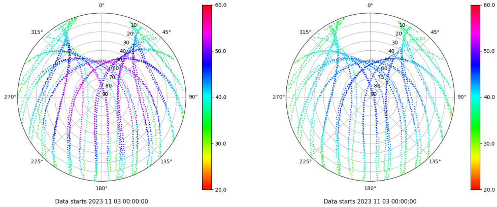
Skyplot for station TAR2. Signal to Noise S1C Data file TAR200ESP_R_2023307.xtr Skyplot for station TAR2. Signal to Noise S2C Data file TAR200ESP_R_2023307.xtr
