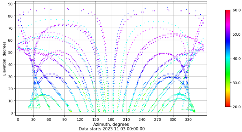
Azimuth-elevation plot for station TAR2. Signal to Noise S1C Data file TAR200ESP_R_2023307.xtr
