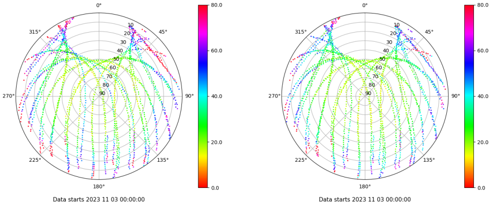
Skyplot for station TAR2. Parameter M1C Data file TAR200ESP_R_2023307.xtr Skyplot for station TAR2. Parameter M2C Data file TAR200ESP_R_2023307.xtr
