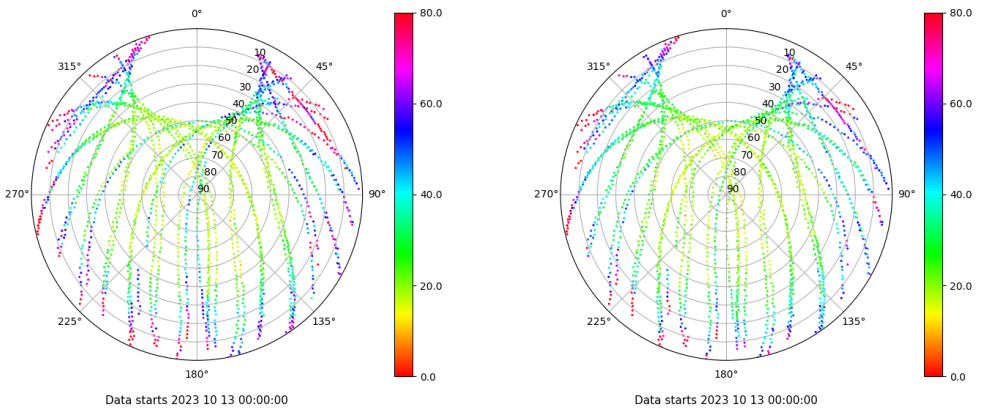
Skyplot for station TAR2. Parameter M1C Data file TAR200ESP_R_2023286.xtr Skyplot for station TAR2. Parameter M2C Data file TAR200ESP_R_2023286.xtr
