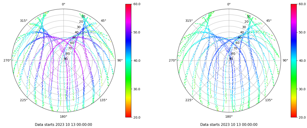
Skyplot for station TAR2. Signal to Noise S1C Data file TAR200ESP_R_2023286.xtr Skyplot for station TAR2. Signal to Noise S2C Data file TAR200ESP_R_2023286.xtr
