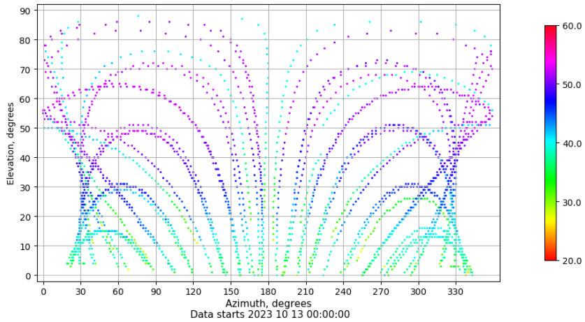
Azimuth-elevation plot for station TAR2. Signal to Noise S1C Data file TAR200ESP_R_2023286.xtr
