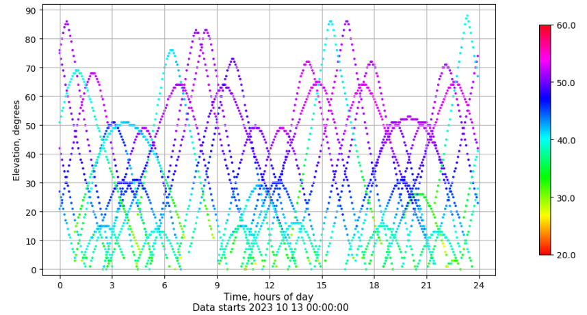
Time-elevation plot for station TAR2. Signal to Noise S1C Data file TAR200ESP_R_2023286.xtr
