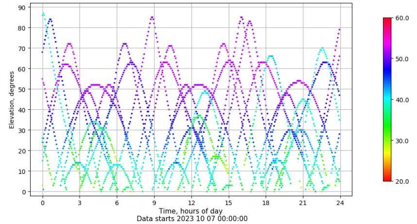
Time-elevation plot for station TAR2. Signal to Noise S1C Data file TAR200ESP_R_2023280.xtr
