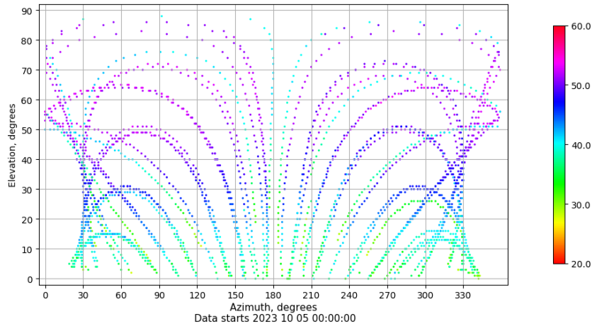
Azimuth-elevation plot for station TAR2. Signal to Noise S1C Data file TAR200ESP_R_2023278.xtr
