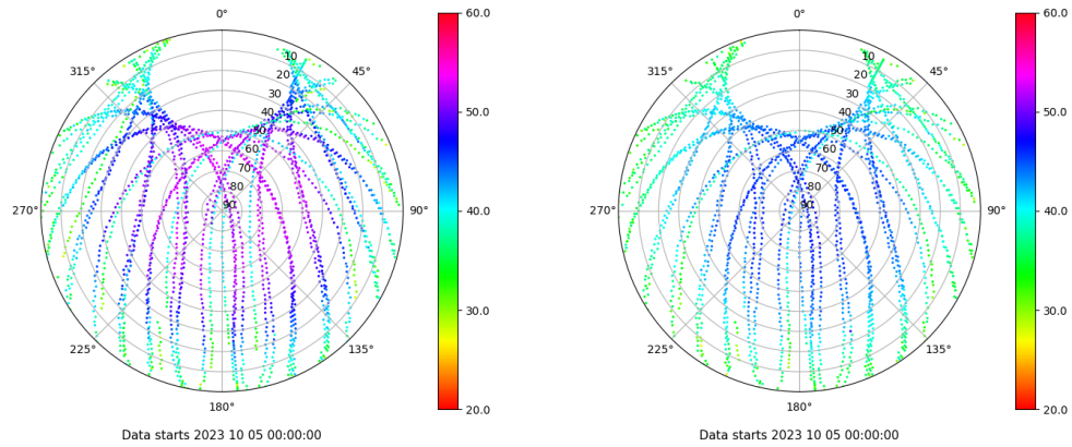
Skyplot for station TAR2. Signal to Noise S1C Data file TAR200ESP_R_2023278.xtr Skyplot for station TAR2. Signal to Noise S2C Data file TAR200ESP_R_2023278.xtr
