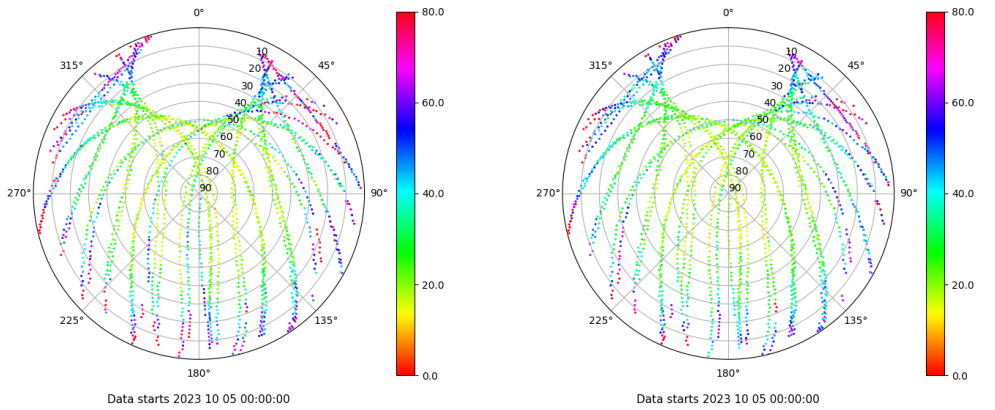
Skyplot for station TAR2. Parameter M1C Data file TAR200ESP_R_2023278.xtr Skyplot for station TAR2. Parameter M2C Data file TAR200ESP_R_2023278.xtr
