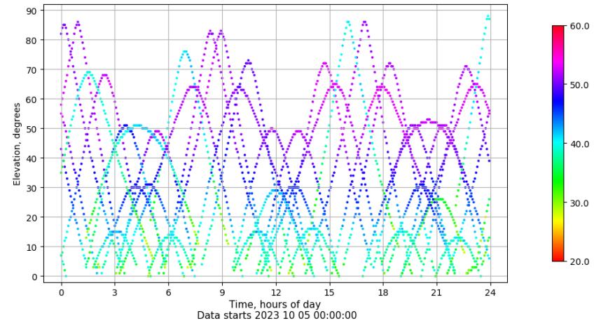
Time-elevation plot for station TAR2. Signal to Noise S1C Data file TAR200ESP_R_2023278.xtr
