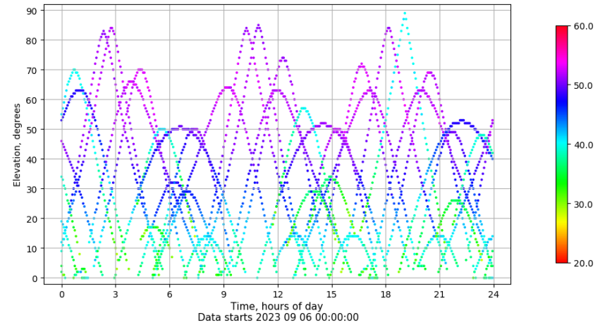
Time-elevation plot for station TAR2. Signal to Noise S1C Data file TAR200ESP_R_2023249.xtr
