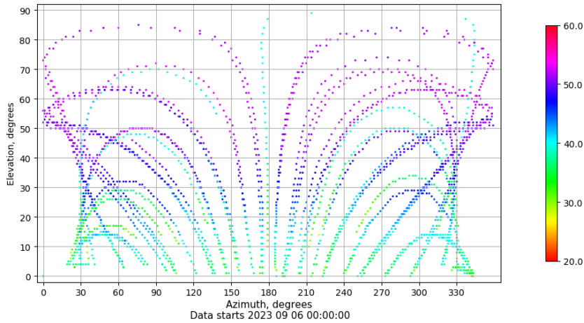
Azimuth-elevation plot for station TAR2. Signal to Noise S1C Data file TAR200ESP_R_2023249.xtr
