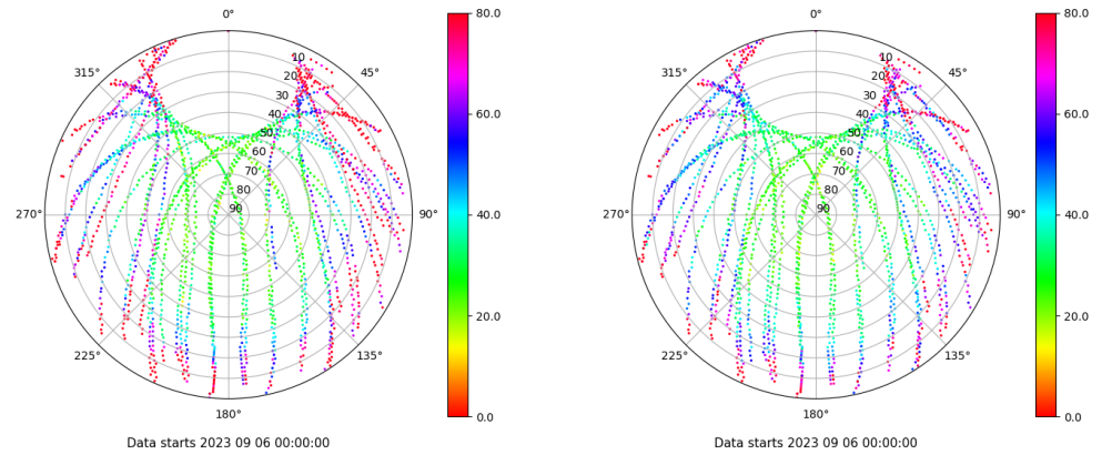
Skyplot for station TAR2. Parameter M1C Data file TAR200ESP_R_2023249.xtr Skyplot for station TAR2. Parameter M2C Data file TAR200ESP_R_2023249.xtr
