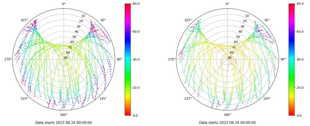
Skyplot for station TAR2. Parameter M1C Data file TAR200ESP_R_2023236.xtr Skyplot for station TAR2. Parameter M2X Data file TAR200ESP_R_2023236.xtr
