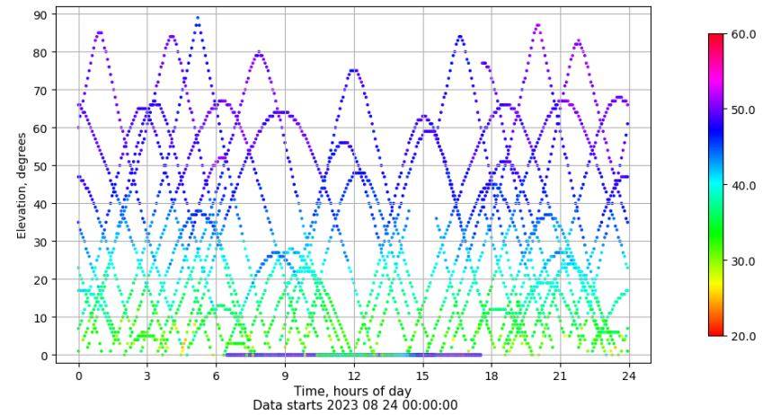
Time-elevation plot for station TAR2. Signal to Noise S1C Data file TAR200ESP_R_2023236.xtr
