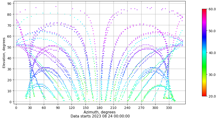
Azimuth-elevation plot for station TAR2. Signal to Noise S1C Data file TAR200ESP_R_2023236.xtr
