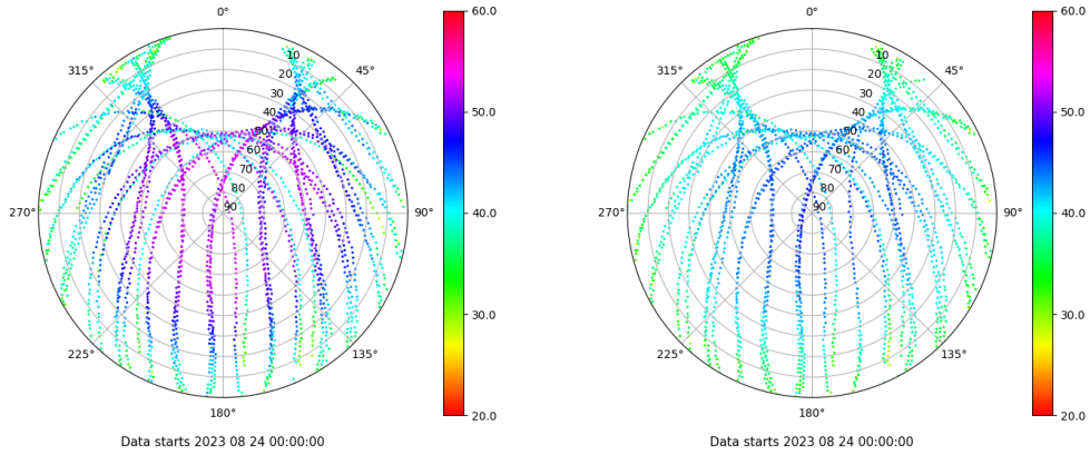
Skyplot for station TAR2. Signal to Noise S1C Data file TAR200ESP_R_2023236.xtr Skyplot for station TAR2. Signal to Noise S2C Data file TAR200ESP_R_2023236.xtr
