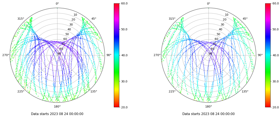
Skyplot for station TAR2. Signal to Noise S1C Data file TAR200ESP_R_2023236.xtr Skyplot for station TAR2. Signal to Noise S2X Data file TAR200ESP_R_2023236.xtr
