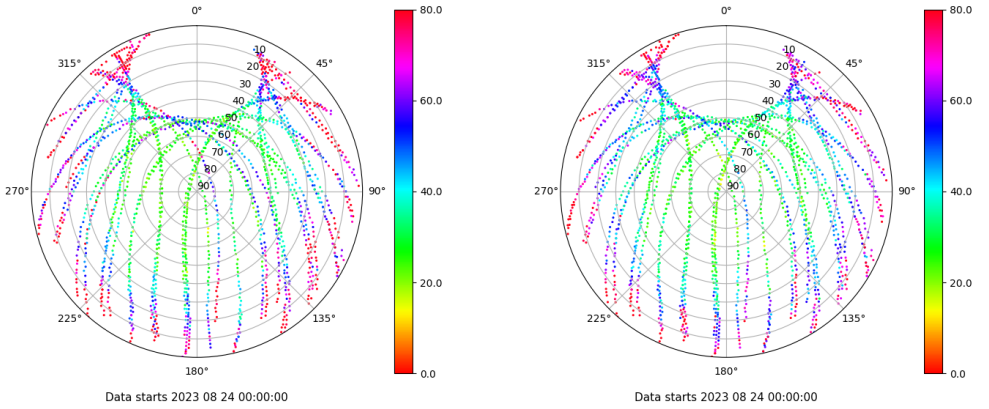
Skyplot for station TAR2. Parameter M1C Data file TAR200ESP_R_2023236.xtr Skyplot for station TAR2. Parameter M2C Data file TAR200ESP_R_2023236.xtr
