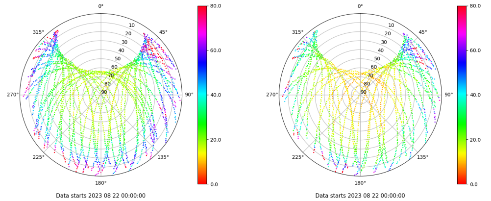
Skyplot for station TAR2. Parameter M1C Data file TAR200ESP_R_2023234.xtr Skyplot for station TAR2. Parameter M2X Data file TAR200ESP_R_2023234.xtr
