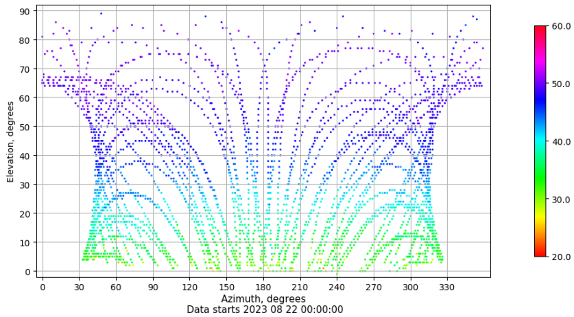
Azimuth-elevation plot for station TAR2. Signal to Noise S1C Data file TAR200ESP_R_2023234.xtr
