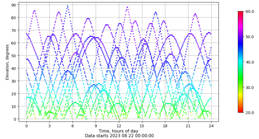
Time-elevation plot for station TAR2. Signal to Noise S1C Data file TAR200ESP_R_2023234.xtr
