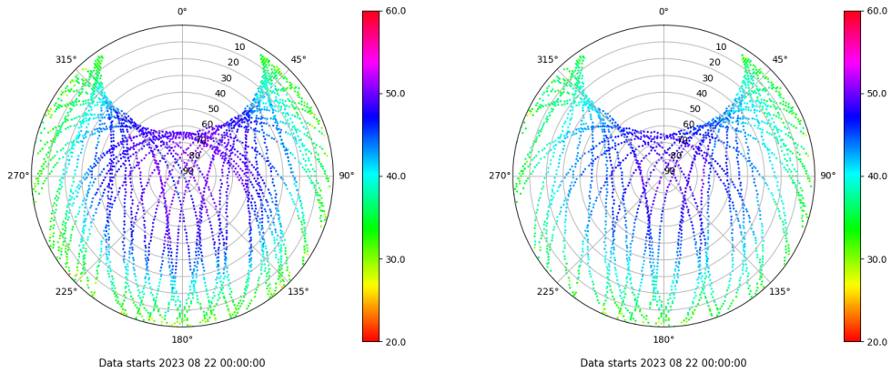
Skyplot for station TAR2. Signal to Noise S1C Data file TAR200ESP_R_2023234.xtr Skyplot for station TAR2. Signal to Noise S2X Data file TAR200ESP_R_2023234.xtr
