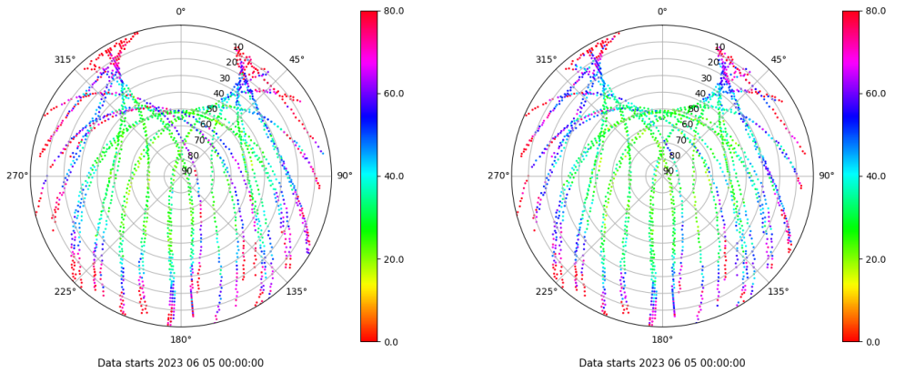
Skyplot for station TAR2. Parameter M1C Data file TAR200ESP_R_2023156.xtr Skyplot for station TAR2. Parameter M2C Data file TAR200ESP_R_2023156.xtr
