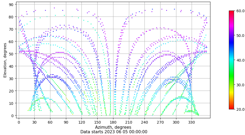
Azimuth-elevation plot for station TAR2. Signal to Noise S1C Data file TAR200ESP_R_2023156.xtr
