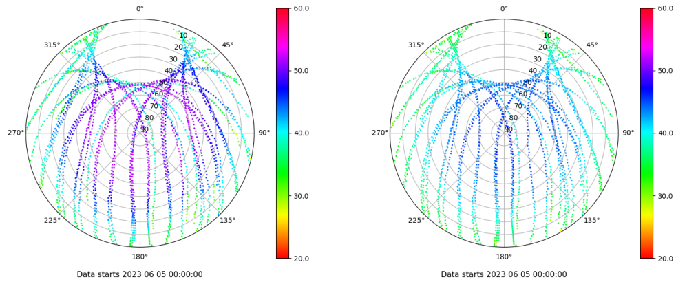
Skyplot for station TAR2. Signal to Noise S1C Data file TAR200ESP_R_2023156.xtr Skyplot for station TAR2. Signal to Noise S2C Data file TAR200ESP_R_2023156.xtr
