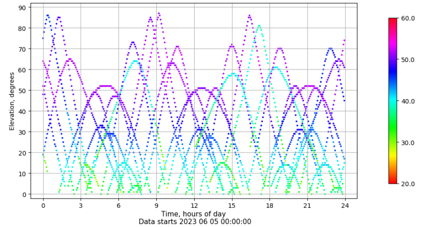
Time-elevation plot for station TAR2. Signal to Noise S1C Data file TAR200ESP_R_2023156.xtr
