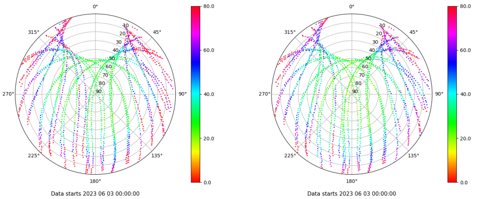
Skyplot for station TAR2. Parameter M1C Data file TAR200ESP_R_2023154.xtr Skyplot for station TAR2. Parameter M2C Data file TAR200ESP_R_2023154.xtr
