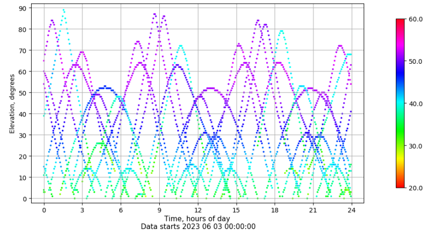
Time-elevation plot for station TAR2. Signal to Noise S1C Data file TAR200ESP_R_2023154.xtr
