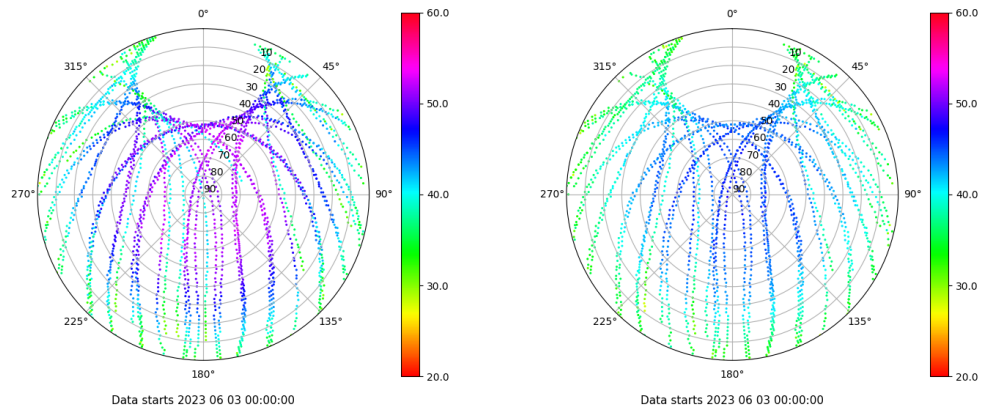
Skyplot for station TAR2. Signal to Noise S1C Data file TAR200ESP_R_2023154.xtr Skyplot for station TAR2. Signal to Noise S2C Data file TAR200ESP_R_2023154.xtr
