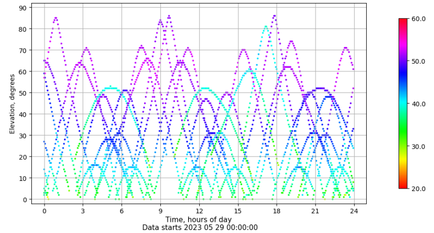
Time-elevation plot for station TAR2. Signal to Noise S1C Data file TAR200ESP_R_2023149.xtr
