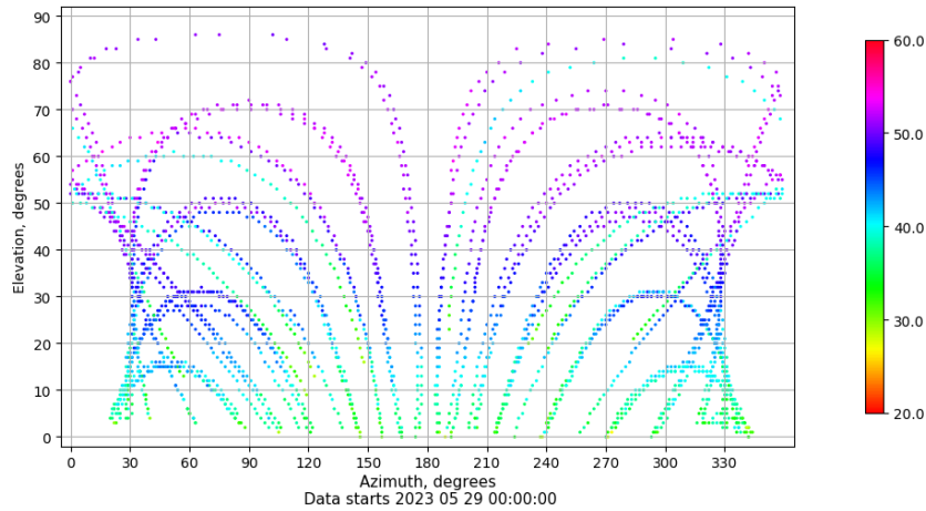
Azimuth-elevation plot for station TAR2. Signal to Noise S1C Data file TAR200ESP_R_2023149.xtr
