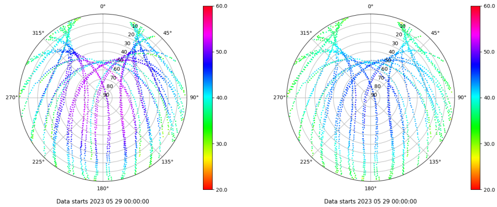
Skyplot for station TAR2. Signal to Noise S1C Data file TAR200ESP_R_2023149.xtr Skyplot for station TAR2. Signal to Noise S2C Data file TAR200ESP_R_2023149.xtr
