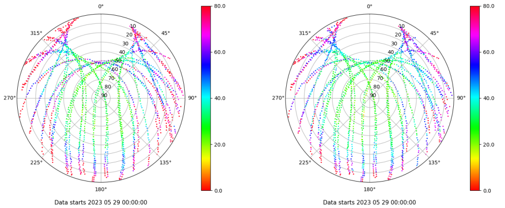
Skyplot for station TAR2. Parameter M1C Data file TAR200ESP_R_2023149.xtr Skyplot for station TAR2. Parameter M2C Data file TAR200ESP_R_2023149.xtr
