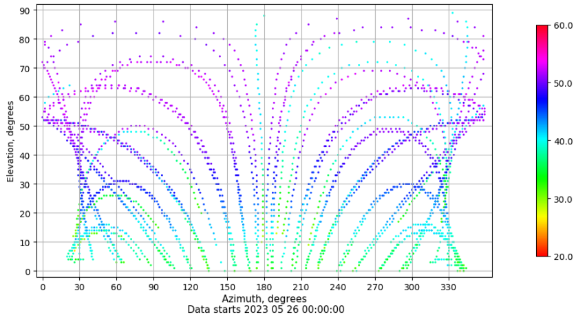
Azimuth-elevation plot for station TAR2. Signal to Noise S1C Data file TAR200ESP_R_2023146.xtr
