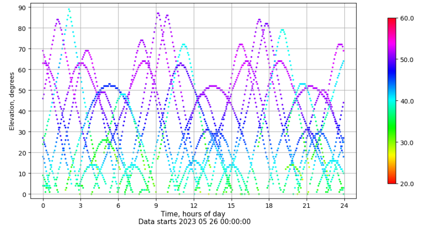
Time-elevation plot for station TAR2. Signal to Noise S1C Data file TAR200ESP_R_2023146.xtr
