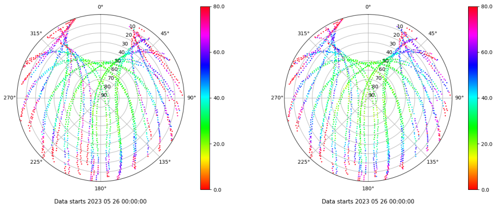
Skyplot for station TAR2. Parameter M1C Data file TAR200ESP_R_2023146.xtr Skyplot for station TAR2. Parameter M2C Data file TAR200ESP_R_2023146.xtr
