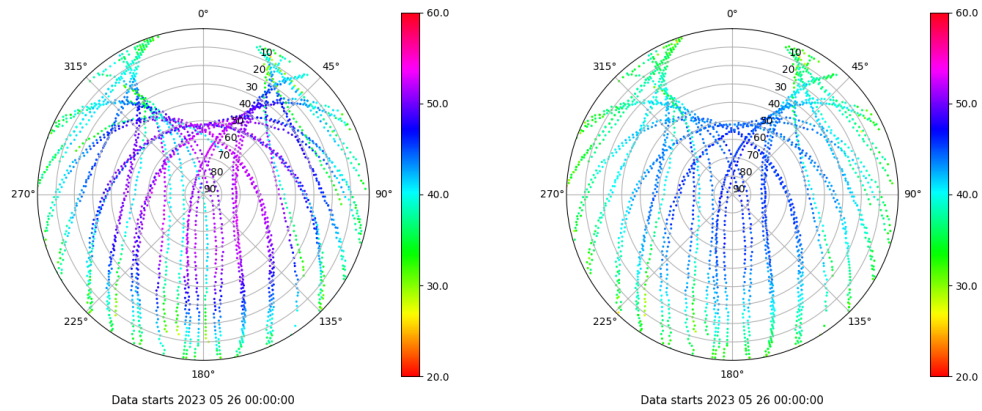
Skyplot for station TAR2. Signal to Noise S1C Data file TAR200ESP_R_2023146.xtr Skyplot for station TAR2. Signal to Noise S2C Data file TAR200ESP_R_2023146.xtr
