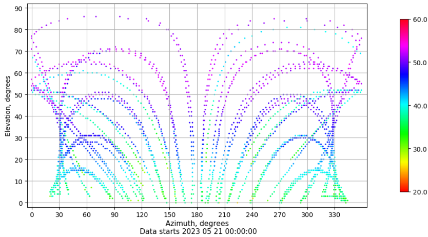
Azimuth-elevation plot for station TAR2. Signal to Noise S1C Data file TAR200ESP_R_2023141.xtr
