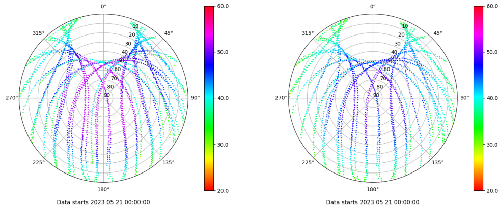
Skyplot for station TAR2. Signal to Noise S1C Data file TAR200ESP_R_2023141.xtr Skyplot for station TAR2. Signal to Noise S2C Data file TAR200ESP_R_2023141.xtr
