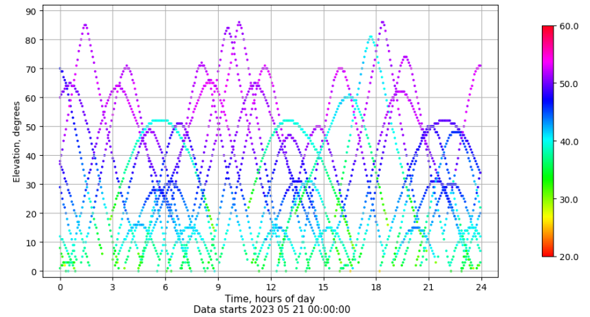
Time-elevation plot for station TAR2. Signal to Noise S1C Data file TAR200ESP_R_2023141.xtr
