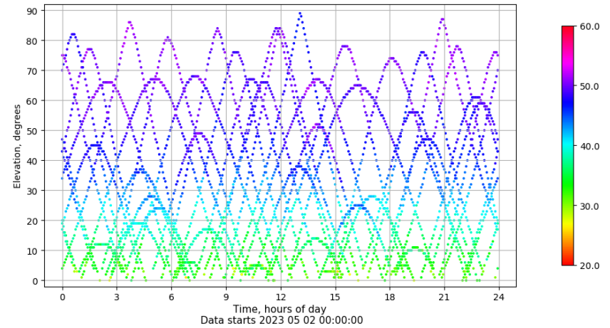
Time-elevation plot for station TAR2. Signal to Noise S1C Data file TAR200ESP_R_2023122.xtr
