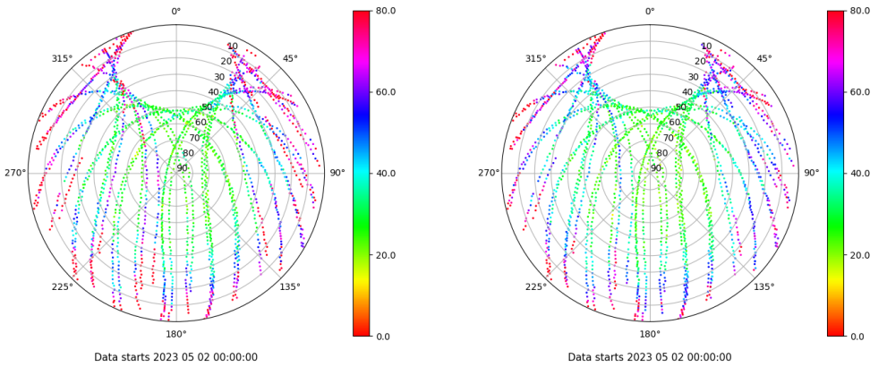
Skyplot for station TAR2. Parameter M1C Data file TAR200ESP_R_2023122.xtr Skyplot for station TAR2. Parameter M2C Data file TAR200ESP_R_2023122.xtr
