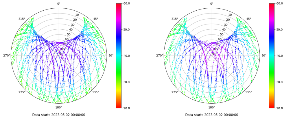
Skyplot for station TAR2. Signal to Noise S1C Data file TAR200ESP_R_2023122.xtr Skyplot for station TAR2. Signal to Noise S2X Data file TAR200ESP_R_2023122.xtr
