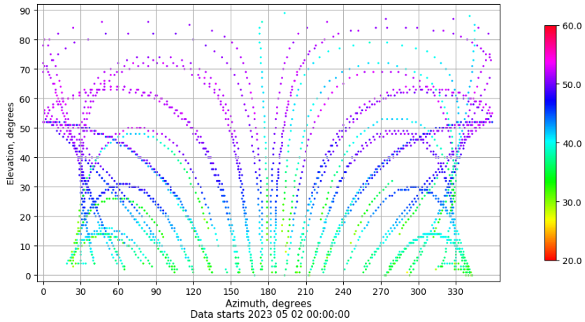
Azimuth-elevation plot for station TAR2. Signal to Noise S1C Data file TAR200ESP_R_2023122.xtr
