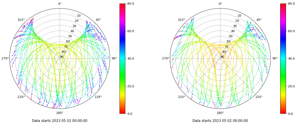
Skyplot for station TAR2. Parameter M1C Data file TAR200ESP_R_2023122.xtr Skyplot for station TAR2. Parameter M2X Data file TAR200ESP_R_2023122.xtr
