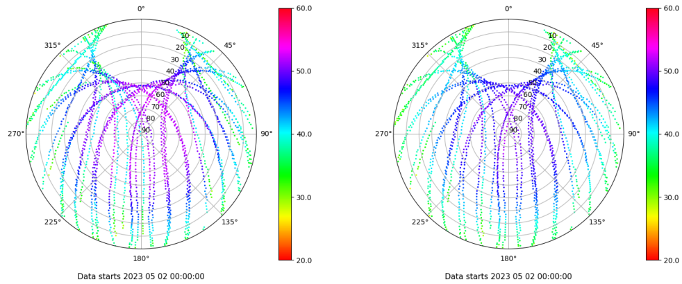
Skyplot for station TAR2. Signal to Noise S1C Data file TAR200ESP_R_2023122.xtr Skyplot for station TAR2. Signal to Noise S2C Data file TAR200ESP_R_2023122.xtr
