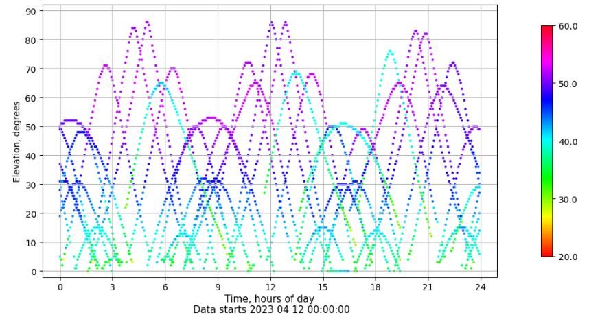
Time-elevation plot for station TAR2. Signal to Noise S1C Data file TAR200ESP_R_2023102.xtr
