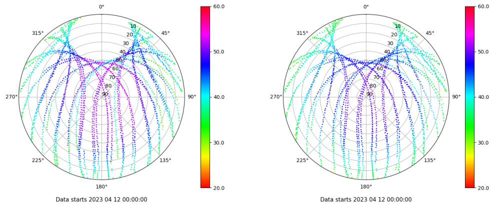
Skyplot for station TAR2. Signal to Noise S1C Data file TAR200ESP_R_2023102.xtr Skyplot for station TAR2. Signal to Noise S2C Data file TAR200ESP_R_2023102.xtr
