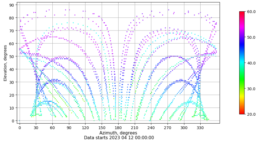
Azimuth-elevation plot for station TAR2. Signal to Noise S1C Data file TAR200ESP_R_2023102.xtr
