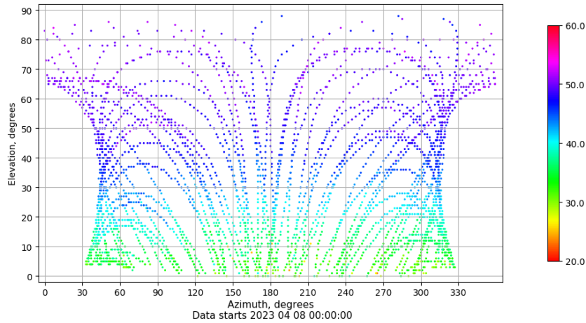
Azimuth-elevation plot for station TAR2. Signal to Noise S1C Data file TAR200ESP_R_2023098.xtr
