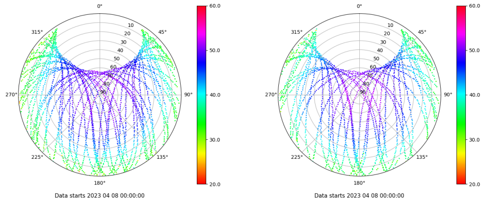
Skyplot for station TAR2. Signal to Noise S1C Data file TAR200ESP_R_2023098.xtr Skyplot for station TAR2. Signal to Noise S2X Data file TAR200ESP_R_2023098.xtr
