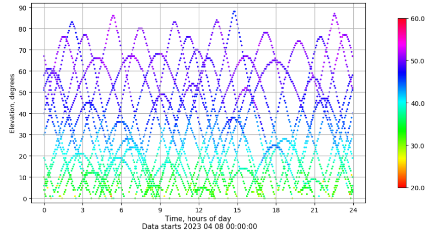
Time-elevation plot for station TAR2. Signal to Noise S1C Data file TAR200ESP_R_2023098.xtr
