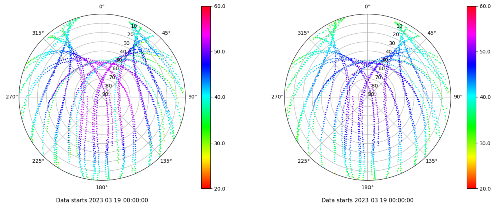
Skyplot for station TAR2. Signal to Noise S1C Data file TAR200ESP_R_2023078.xtr Skyplot for station TAR2. Signal to Noise S2C Data file TAR200ESP_R_2023078.xtr
