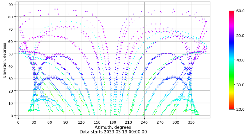
Azimuth-elevation plot for station TAR2. Signal to Noise S1C Data file TAR200ESP_R_2023078.xtr
