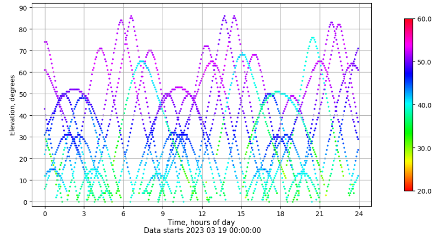
Time-elevation plot for station TAR2. Signal to Noise S1C Data file TAR200ESP_R_2023078.xtr
