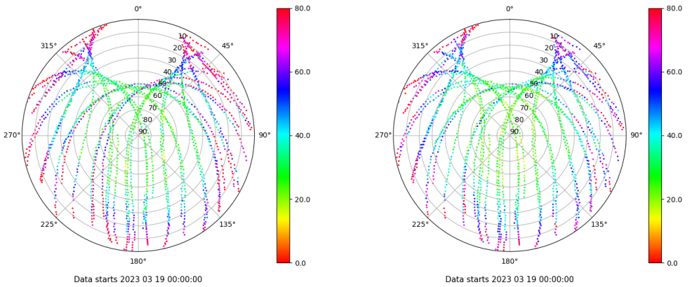
Skyplot for station TAR2. Parameter M1C Data file TAR200ESP_R_2023078.xtr Skyplot for station TAR2. Parameter M2C Data file TAR200ESP_R_2023078.xtr
