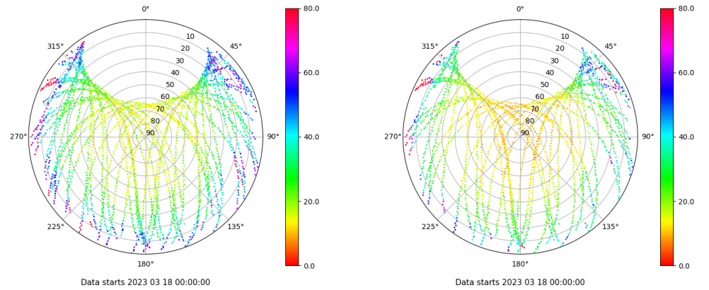
Skyplot for station TAR2. Parameter M1C Data file TAR200ESP_R_2023077.xtr Skyplot for station TAR2. Parameter M2X Data file TAR200ESP_R_2023077.xtr
