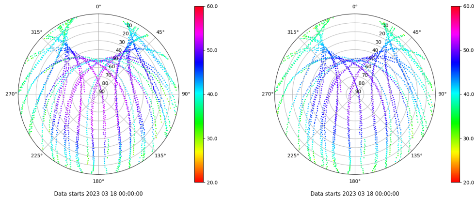
Skyplot for station TAR2. Signal to Noise S1C Data file TAR200ESP_R_2023077.xtr Skyplot for station TAR2. Signal to Noise S2C Data file TAR200ESP_R_2023077.xtr
