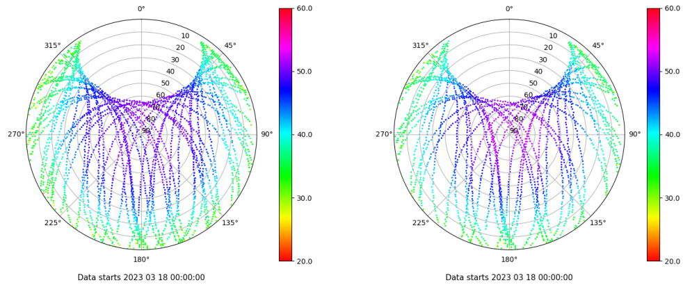
Skyplot for station TAR2. Signal to Noise S1C Data file TAR200ESP_R_2023077.xtr Skyplot for station TAR2. Signal to Noise S2X Data file TAR200ESP_R_2023077.xtr
