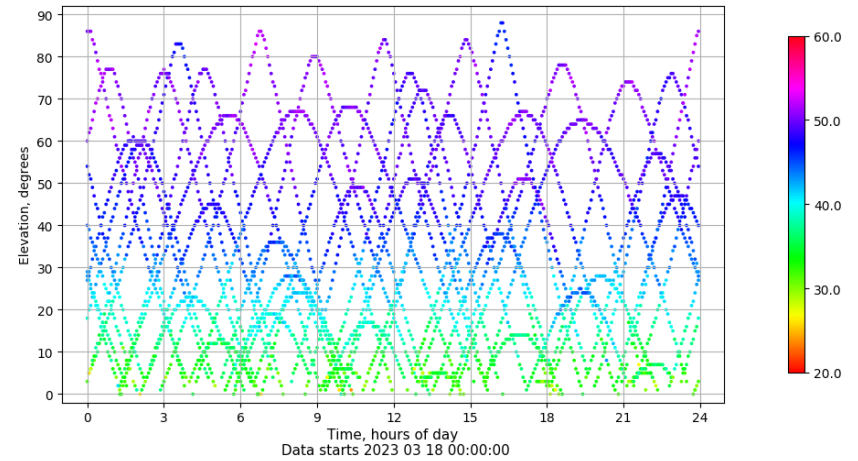
Time-elevation plot for station TAR2. Signal to Noise S1C Data file TAR200ESP_R_2023077.xtr
