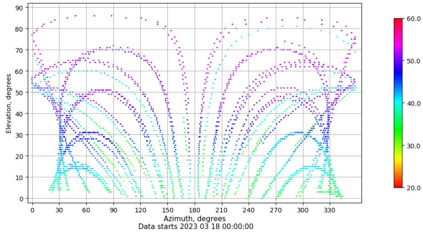
Azimuth-elevation plot for station TAR2. Signal to Noise S1C Data file TAR200ESP_R_2023077.xtr
