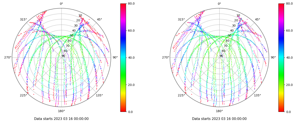
Skyplot for station TAR2. Parameter M1C Data file TAR200ESP_R_2023075.xtr Skyplot for station TAR2. Parameter M2C Data file TAR200ESP_R_2023075.xtr
