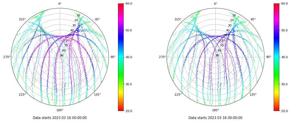
Skyplot for station TAR2. Signal to Noise S1C Data file TAR200ESP_R_2023075.xtr Skyplot for station TAR2. Signal to Noise S2C Data file TAR200ESP_R_2023075.xtr
