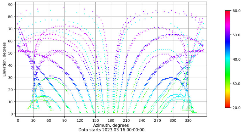
Azimuth-elevation plot for station TAR2. Signal to Noise S1C Data file TAR200ESP_R_2023075.xtr
