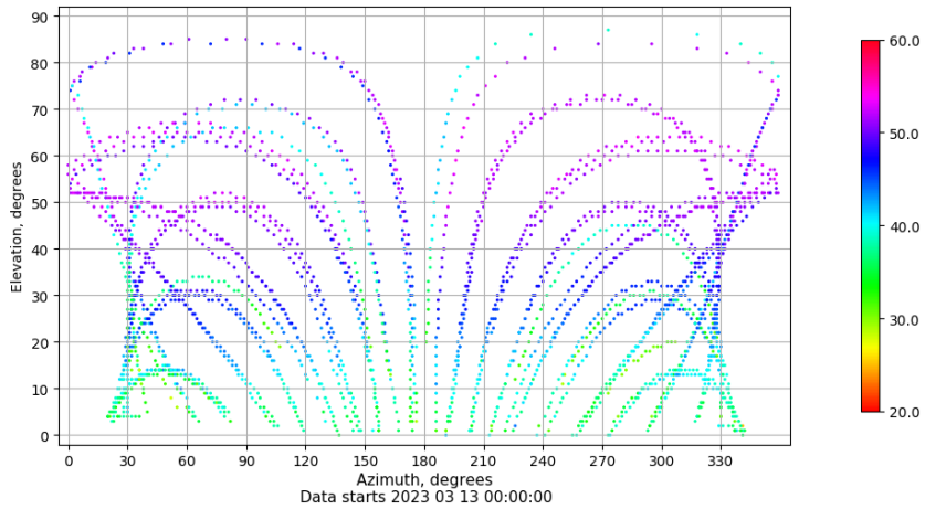
Azimuth-elevation plot for station TAR2. Signal to Noise S1C Data file TAR200ESP_R_2023072.xtr
