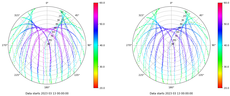
Skyplot for station TAR2. Signal to Noise S1C Data file TAR200ESP_R_2023072.xtr Skyplot for station TAR2. Signal to Noise S2C Data file TAR200ESP_R_2023072.xtr
