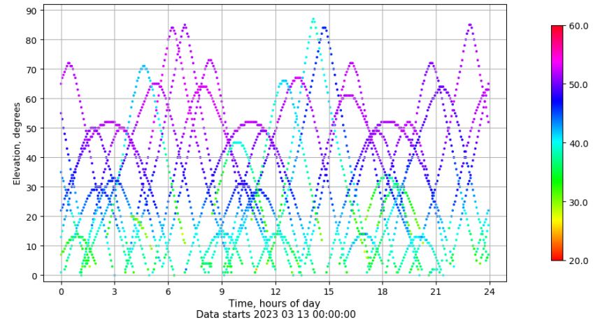
Time-elevation plot for station TAR2. Signal to Noise S1C Data file TAR200ESP_R_2023072.xtr
