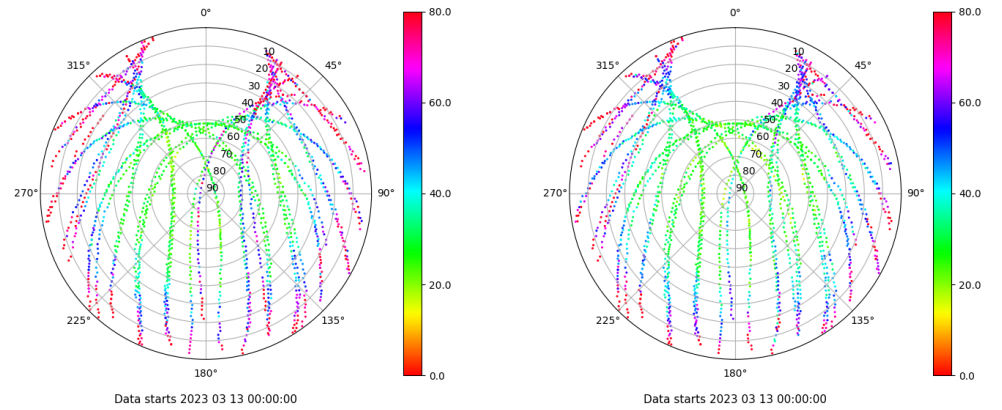
Skyplot for station TAR2. Parameter M1C Data file TAR200ESP_R_2023072.xtr Skyplot for station TAR2. Parameter M2C Data file TAR200ESP_R_2023072.xtr
