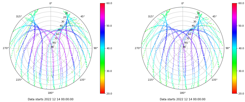
Skyplot for station TAR2. Signal to Noise S1C Data file TAR200ESP_R_2022348.xtr Skyplot for station TAR2. Signal to Noise S2C Data file TAR200ESP_R_2022348.xtr
