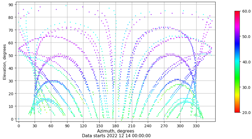
Azimuth-elevation plot for station TAR2. Signal to Noise S1C Data file TAR200ESP_R_2022348.xtr
