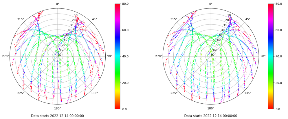
Skyplot for station TAR2. Parameter M1C Data file TAR200ESP_R_2022348.xtr Skyplot for station TAR2. Parameter M2C Data file TAR200ESP_R_2022348.xtr
