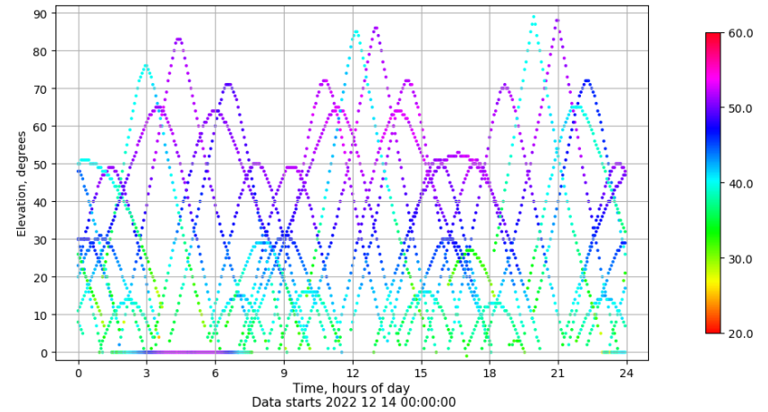
Time-elevation plot for station TAR2. Signal to Noise S1C Data file TAR200ESP_R_2022348.xtr
