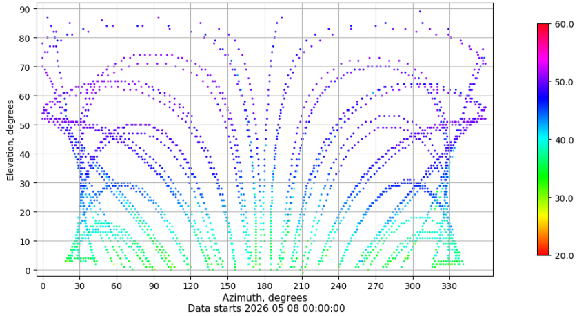
Azimuth-elevation plot for station TAR0. Signal to Noise S1C Data file TAR000ESP_R_2026128.xtr
