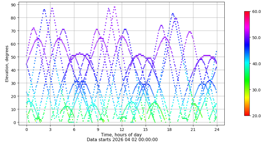
Time-elevation plot for station TAR0. Signal to Noise S1C Data file TAR000ESP_R_2026092.xtr
