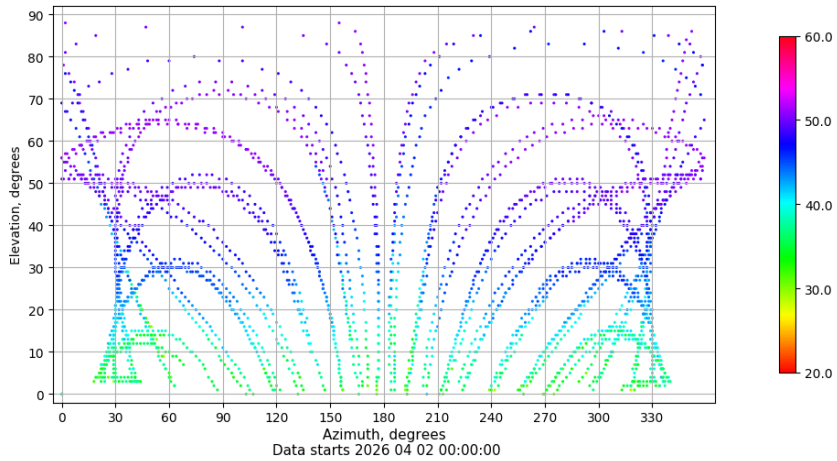
Azimuth-elevation plot for station TAR0. Signal to Noise S1C Data file TAR000ESP_R_2026092.xtr
