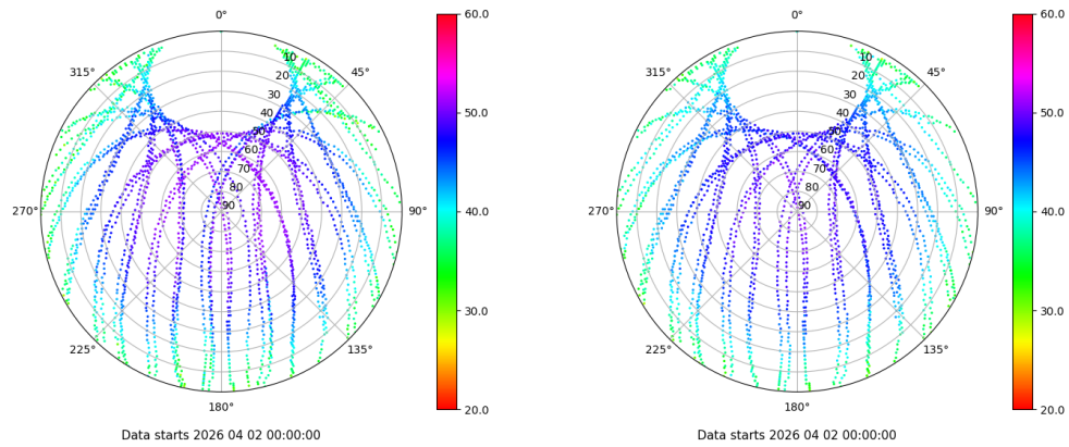
Skyplot for station TAR0. Signal to Noise S1C Data file TAR000ESP_R_2026092.xtr Skyplot for station TAR0. Signal to Noise S2P Data file TAR000ESP_R_2026092.xtr
