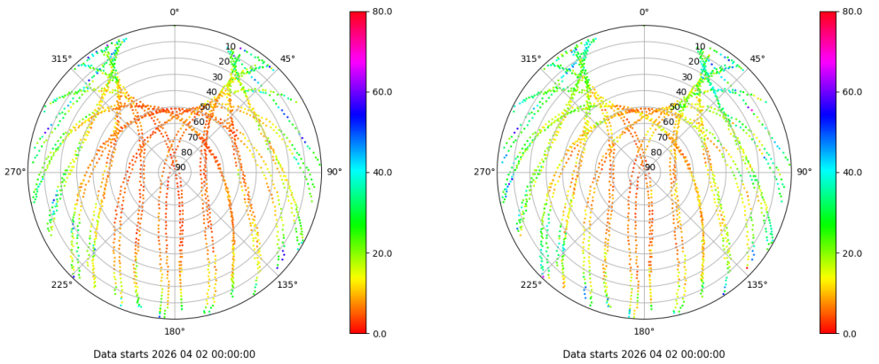
Skyplot for station TAR0. Parameter M1C Data file TAR000ESP_R_2026092.xtr Skyplot for station TAR0. Parameter M2P Data file TAR000ESP_R_2026092.xtr
