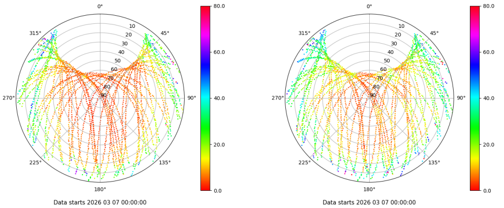
Skyplot for station TAR0. Parameter M1C Data file TAR000ESP_R_2026066.xtr Skyplot for station TAR0. Parameter M2W Data file TAR000ESP_R_2026066.xtr
