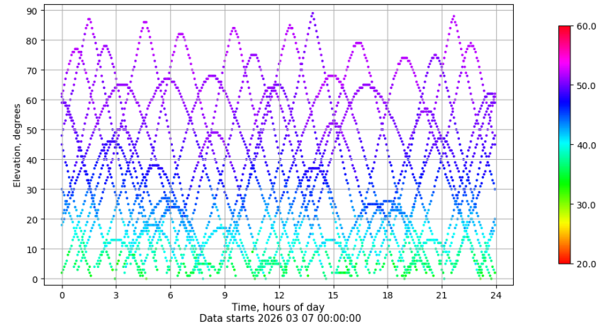
Time-elevation plot for station TAR0. Signal to Noise S1C Data file TAR000ESP_R_2026066.xtr
