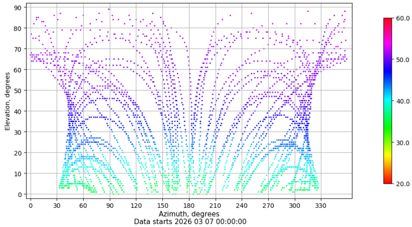
Azimuth-elevation plot for station TAR0. Signal to Noise S1C Data file TAR000ESP_R_2026066.xtr
