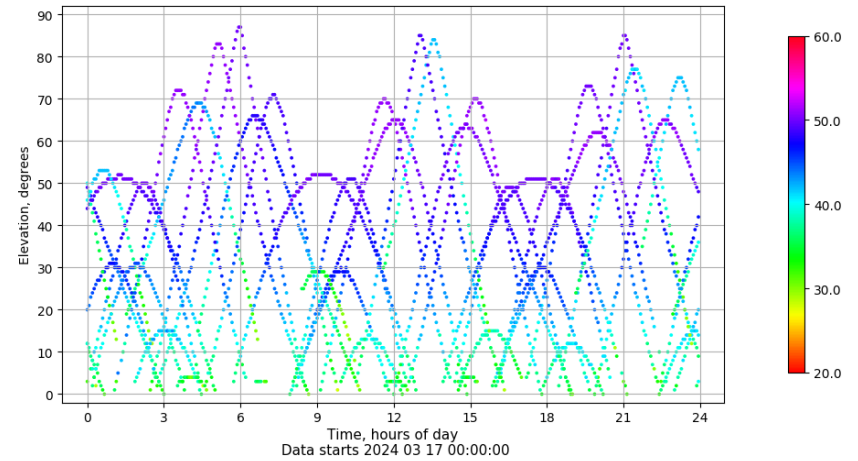
Time-elevation plot for station TAR0. Signal to Noise S1C Data file TAR000ESP_R_2024077.xtr
