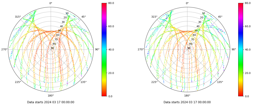
Skyplot for station TAR0. Parameter M1C Data file TAR000ESP_R_2024077.xtr Skyplot for station TAR0. Parameter M2P Data file TAR000ESP_R_2024077.xtr
