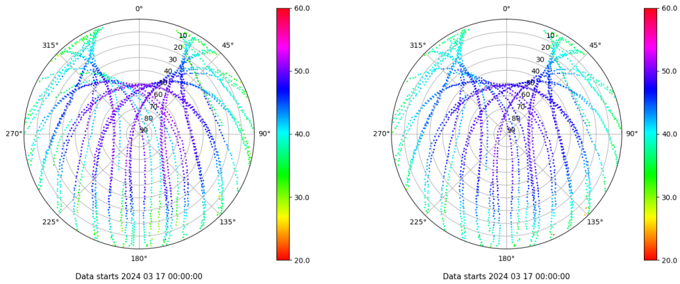
Skyplot for station TAR0. Signal to Noise S1C Data file TAR000ESP_R_2024077.xtr Skyplot for station TAR0. Signal to Noise S2P Data file TAR000ESP_R_2024077.xtr
