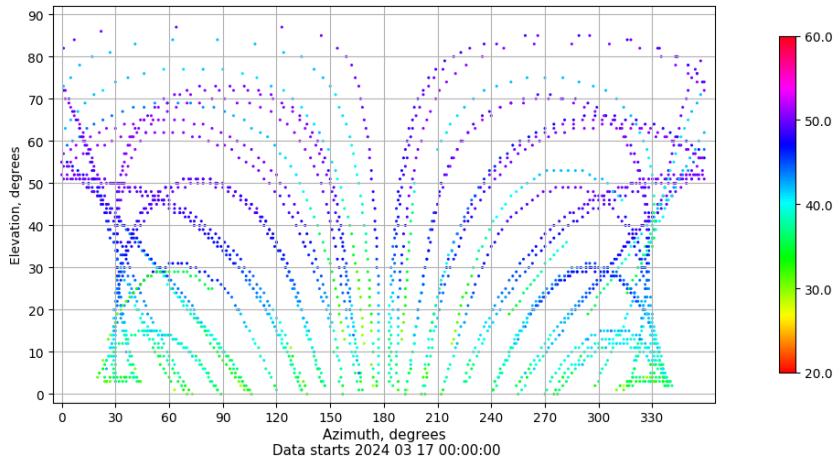
Azimuth-elevation plot for station TAR0. Signal to Noise S1C Data file TAR000ESP_R_2024077.xtr
