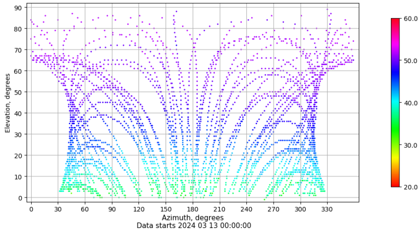
Azimuth-elevation plot for station TAR0. Signal to Noise S1C Data file TAR000ESP_R_2024073.xtr
