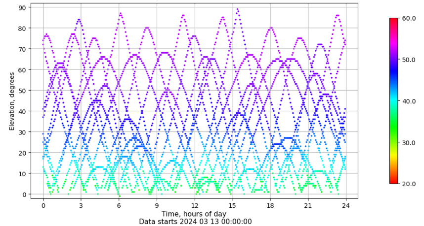
Time-elevation plot for station TAR0. Signal to Noise S1C Data file TAR000ESP_R_2024073.xtr
