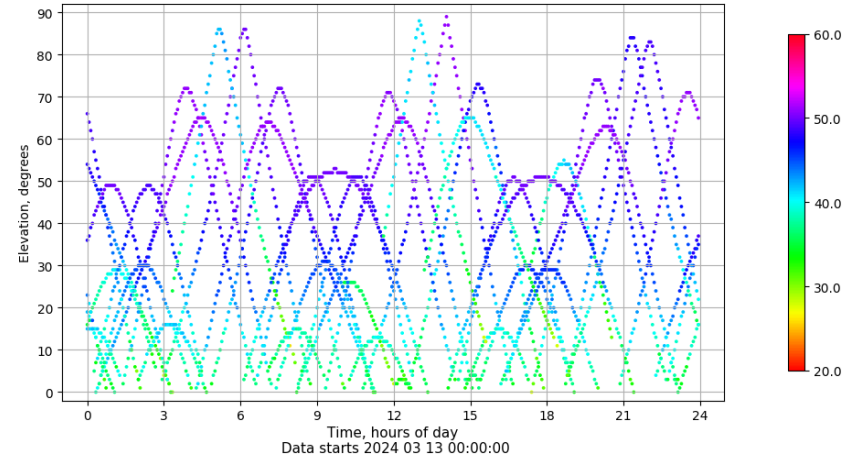
Time-elevation plot for station TAR0. Signal to Noise S1C Data file TAR000ESP_R_2024073.xtr
