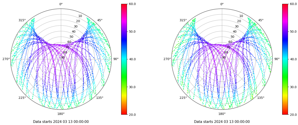
Skyplot for station TAR0. Signal to Noise S1C Data file TAR000ESP_R_2024073.xtr Skyplot for station TAR0. Signal to Noise S2W Data file TAR000ESP_R_2024073.xtr
