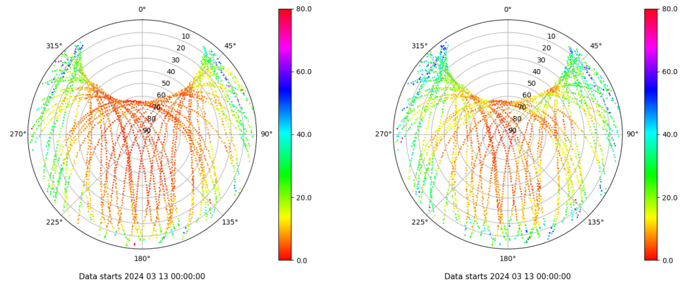
Skyplot for station TAR0. Parameter M1C Data file TAR000ESP_R_2024073.xtr Skyplot for station TAR0. Parameter M2W Data file TAR000ESP_R_2024073.xtr
