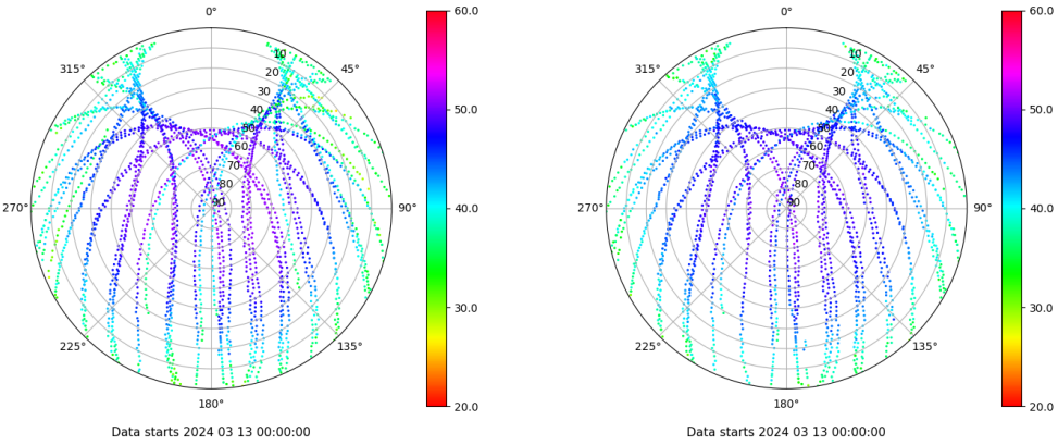
Skyplot for station TAR0. Signal to Noise S1C Data file TAR000ESP_R_2024073.xtr Skyplot for station TAR0. Signal to Noise S2P Data file TAR000ESP_R_2024073.xtr
