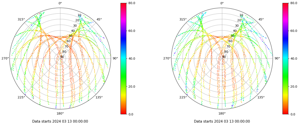
Skyplot for station TAR0. Parameter M1C Data file TAR000ESP_R_2024073.xtr Skyplot for station TAR0. Parameter M2P Data file TAR000ESP_R_2024073.xtr
