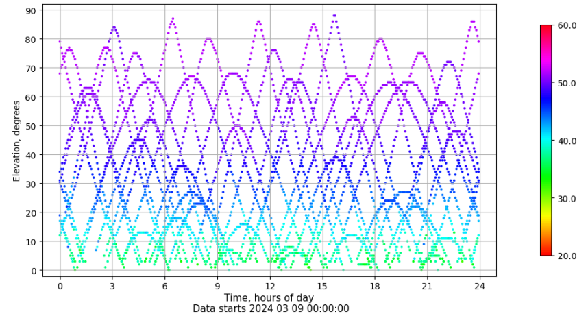
Time-elevation plot for station TAR0. Signal to Noise S1C Data file TAR000ESP_R_2024069.xtr
