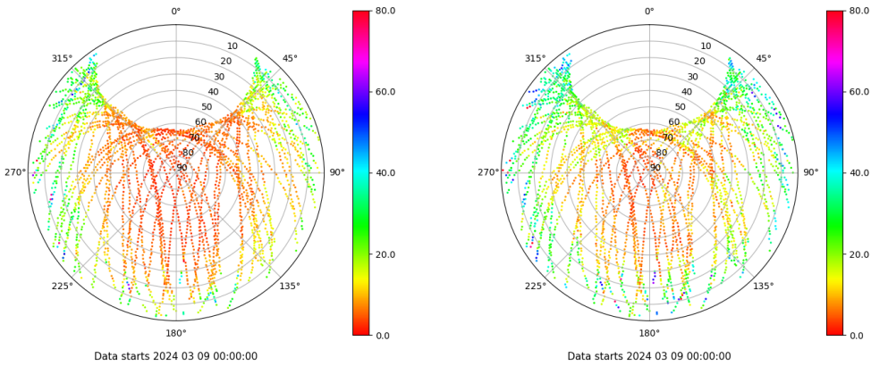
Skyplot for station TAR0. Parameter M1C Data file TAR000ESP_R_2024069.xtr Skyplot for station TAR0. Parameter M2W Data file TAR000ESP_R_2024069.xtr
