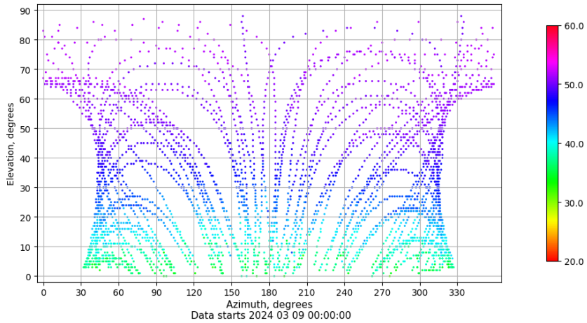
Azimuth-elevation plot for station TAR0. Signal to Noise S1C Data file TAR000ESP_R_2024069.xtr
