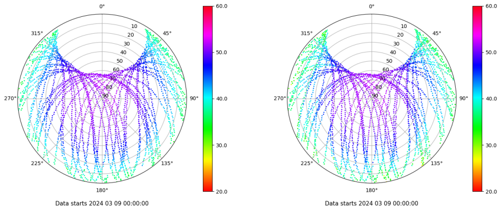
Skyplot for station TAR0. Signal to Noise S1C Data file TAR000ESP_R_2024069.xtr Skyplot for station TAR0. Signal to Noise S2W Data file TAR000ESP_R_2024069.xtr
