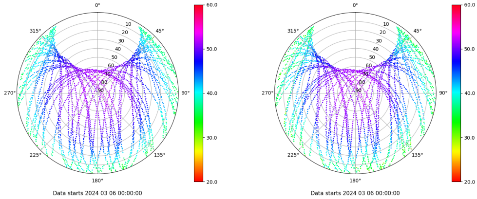
Skyplot for station TAR0. Signal to Noise S1C Data file TAR000ESP_R_2024066.xtr Skyplot for station TAR0. Signal to Noise S2W Data file TAR000ESP_R_2024066.xtr
