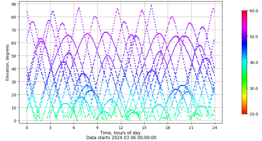
Time-elevation plot for station TAR0. Signal to Noise S1C Data file TAR000ESP_R_2024066.xtr
