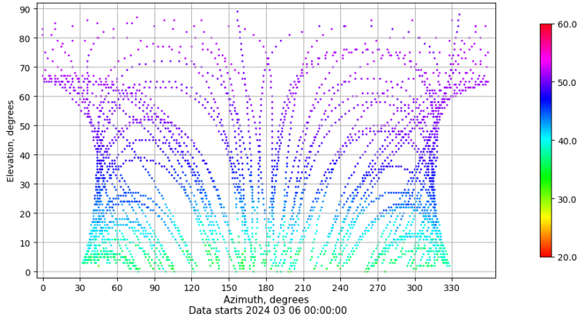
Azimuth-elevation plot for station TAR0. Signal to Noise S1C Data file TAR000ESP_R_2024066.xtr
