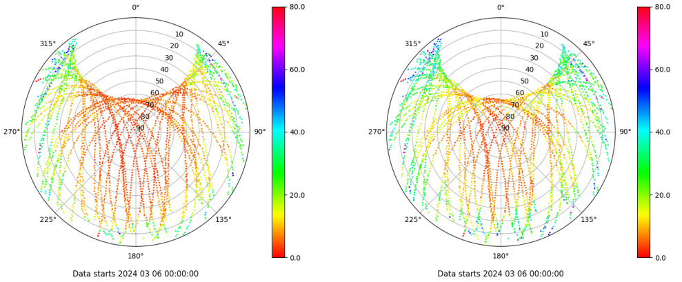
Skyplot for station TAR0. Parameter M1C Data file TAR000ESP_R_2024066.xtr Skyplot for station TAR0. Parameter M2W Data file TAR000ESP_R_2024066.xtr
