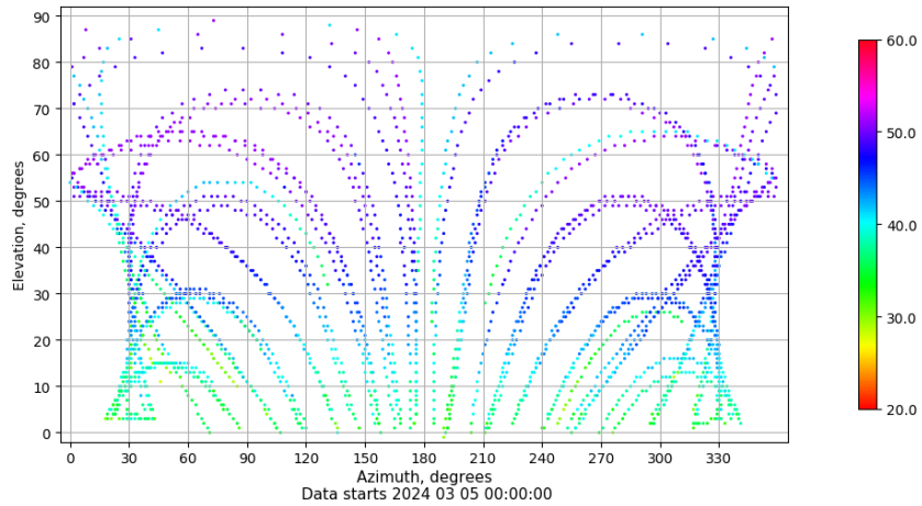
Azimuth-elevation plot for station TAR0. Signal to Noise S1C Data file TAR000ESP_R_2024065.xtr
