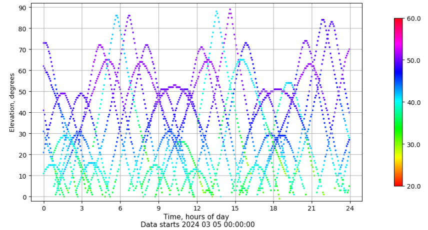
Time-elevation plot for station TAR0. Signal to Noise S1C Data file TAR000ESP_R_2024065.xtr
