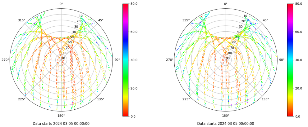
Skyplot for station TAR0. Parameter M1C Data file TAR000ESP_R_2024065.xtr Skyplot for station TAR0. Parameter M2P Data file TAR000ESP_R_2024065.xtr
