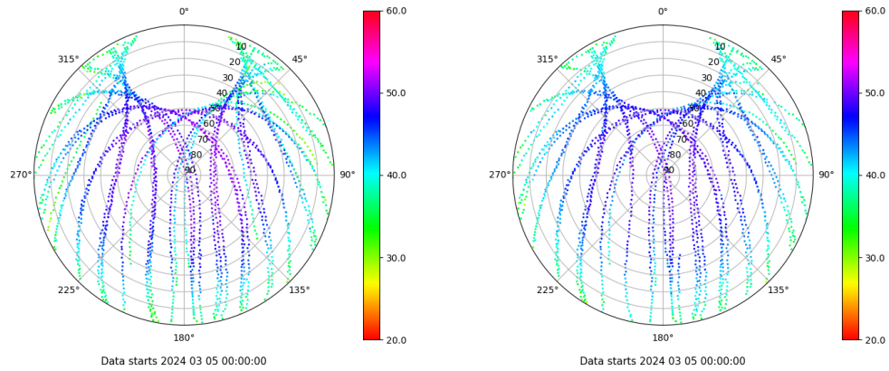
Skyplot for station TAR0. Signal to Noise S1C Data file TAR000ESP_R_2024065.xtr Skyplot for station TAR0. Signal to Noise S2P Data file TAR000ESP_R_2024065.xtr
