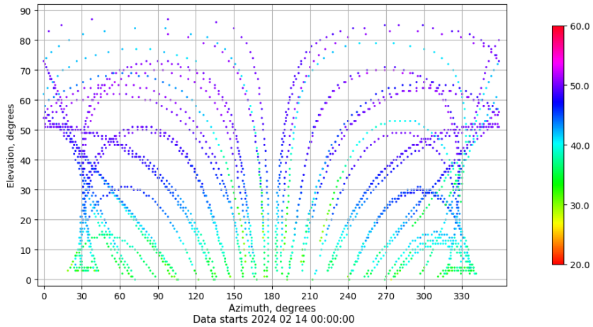
Azimuth-elevation plot for station TAR0. Signal to Noise S1C Data file TAR000ESP_R_2024045.xtr
