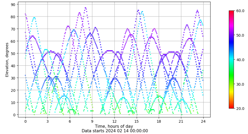
Time-elevation plot for station TAR0. Signal to Noise S1C Data file TAR000ESP_R_2024045.xtr
