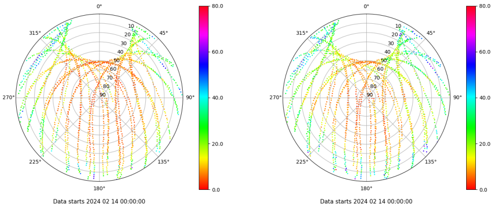
Skyplot for station TAR0. Parameter M1C Data file TAR000ESP_R_2024045.xtr Skyplot for station TAR0. Parameter M2P Data file TAR000ESP_R_2024045.xtr
