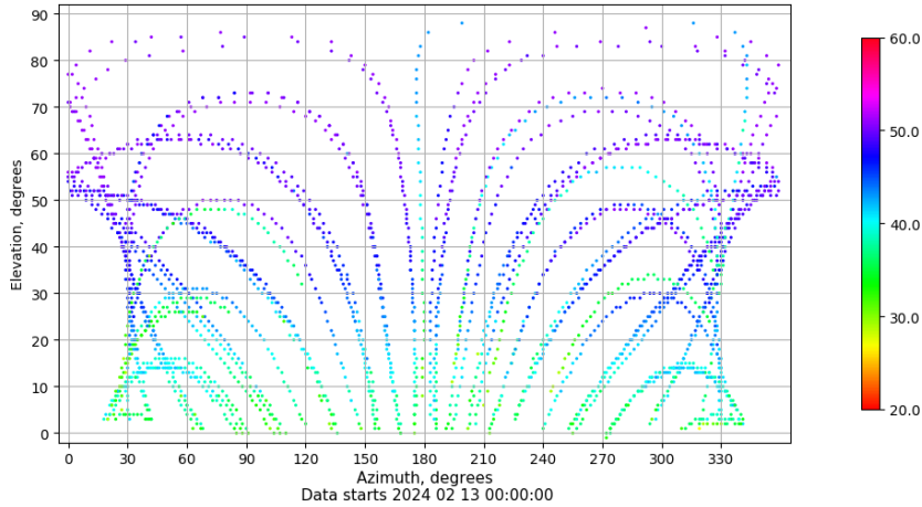
Azimuth-elevation plot for station TAR0. Signal to Noise S1C Data file TAR000ESP_R_2024044.xtr
