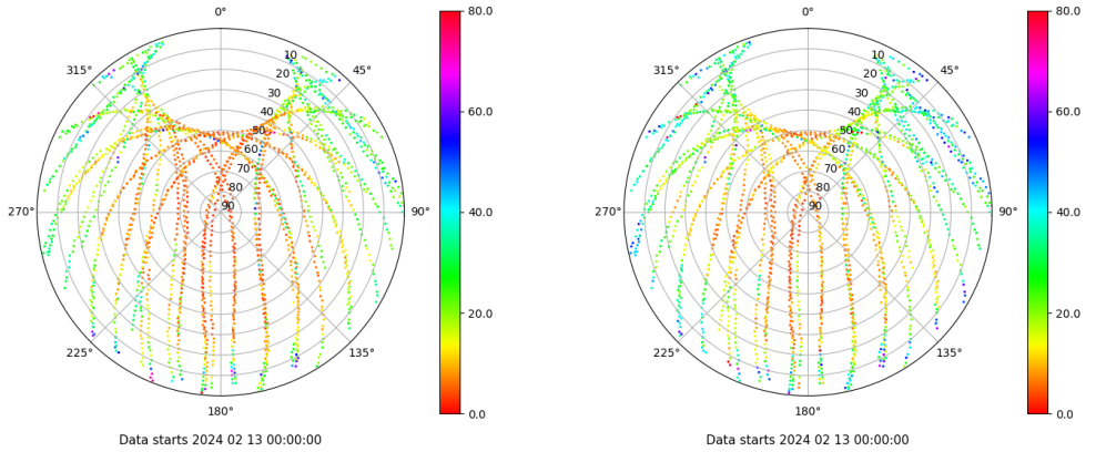
Skyplot for station TAR0. Parameter M1C Data file TAR000ESP_R_2024044.xtr Skyplot for station TAR0. Parameter M2P Data file TAR000ESP_R_2024044.xtr
