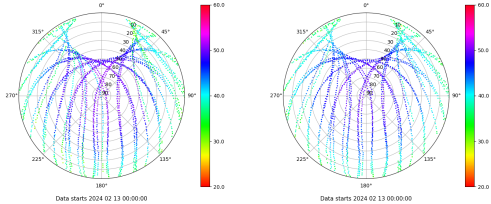
Skyplot for station TAR0. Signal to Noise S1C Data file TAR000ESP_R_2024044.xtr Skyplot for station TAR0. Signal to Noise S2P Data file TAR000ESP_R_2024044.xtr
