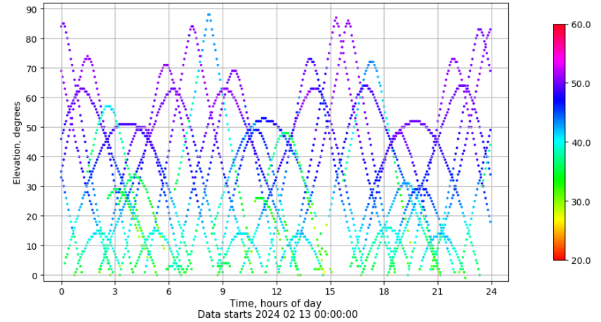
Time-elevation plot for station TAR0. Signal to Noise S1C Data file TAR000ESP_R_2024044.xtr
