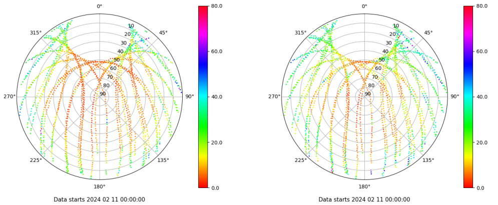
Skyplot for station TAR0. Parameter M1C Data file TAR000ESP_R_2024042.xtr Skyplot for station TAR0. Parameter M2P Data file TAR000ESP_R_2024042.xtr
