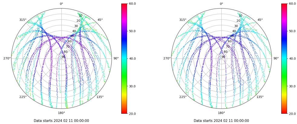
Skyplot for station TAR0. Signal to Noise S1C Data file TAR000ESP_R_2024042.xtr Skyplot for station TAR0. Signal to Noise S2P Data file TAR000ESP_R_2024042.xtr
