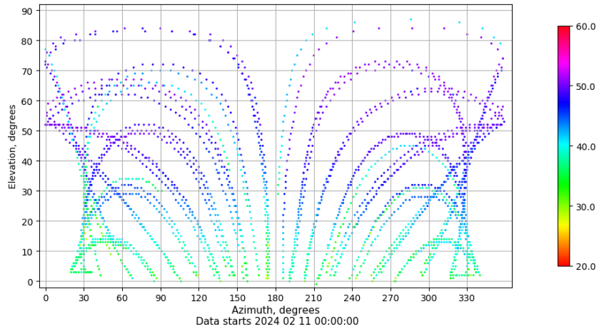
Azimuth-elevation plot for station TAR0. Signal to Noise S1C Data file TAR000ESP_R_2024042.xtr
