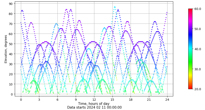
Time-elevation plot for station TAR0. Signal to Noise S1C Data file TAR000ESP_R_2024042.xtr
