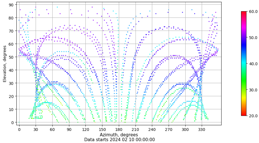
Azimuth-elevation plot for station TAR0. Signal to Noise S1C Data file TAR000ESP_R_2024041.xtr
