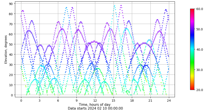
Time-elevation plot for station TAR0. Signal to Noise S1C Data file TAR000ESP_R_2024041.xtr
