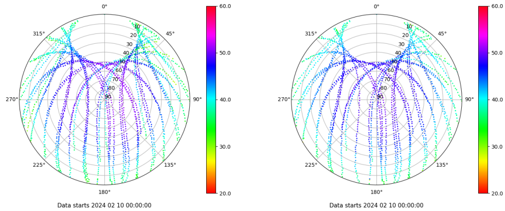
Skyplot for station TAR0. Signal to Noise S1C Data file TAR000ESP_R_2024041.xtr Skyplot for station TAR0. Signal to Noise S2P Data file TAR000ESP_R_2024041.xtr
