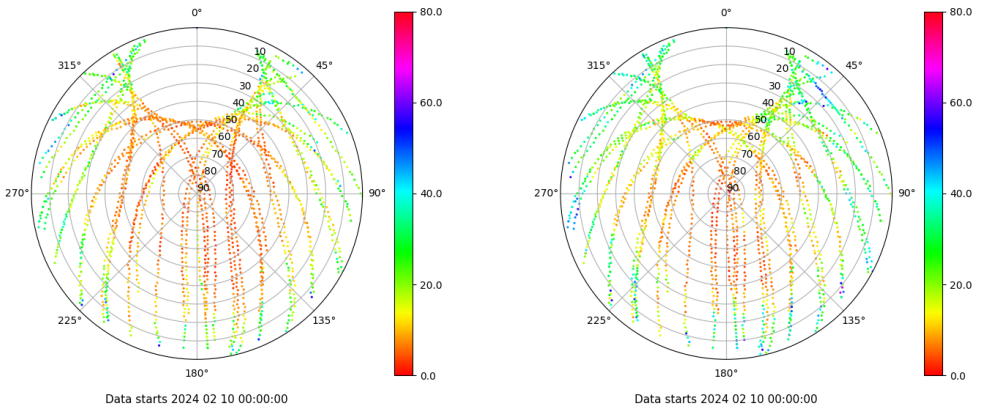
Skyplot for station TAR0. Parameter M1C Data file TAR000ESP_R_2024041.xtr Skyplot for station TAR0. Parameter M2P Data file TAR000ESP_R_2024041.xtr
