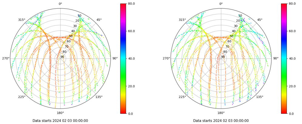
Skyplot for station TAR0. Parameter M1C Data file TAR000ESP_R_2024034.xtr Skyplot for station TAR0. Parameter M2P Data file TAR000ESP_R_2024034.xtr
