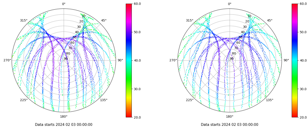
Skyplot for station TAR0. Signal to Noise S1C Data file TAR000ESP_R_2024034.xtr Skyplot for station TAR0. Signal to Noise S2P Data file TAR000ESP_R_2024034.xtr
