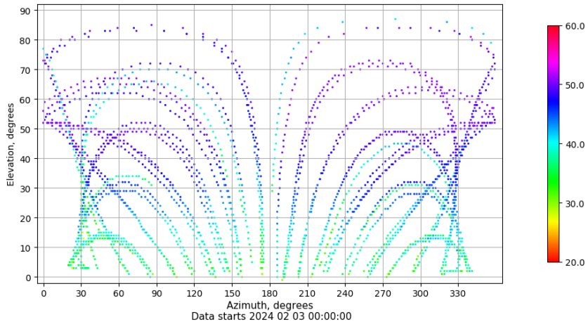
Azimuth-elevation plot for station TAR0. Signal to Noise S1C Data file TAR000ESP_R_2024034.xtr
