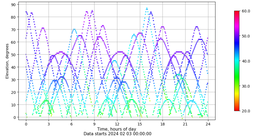
Time-elevation plot for station TAR0. Signal to Noise S1C Data file TAR000ESP_R_2024034.xtr
