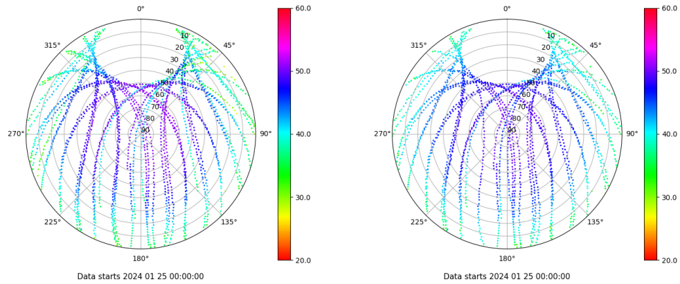
Skyplot for station TAR0. Signal to Noise S1C Data file TAR000ESP_R_2024025.xtr Skyplot for station TAR0. Signal to Noise S2P Data file TAR000ESP_R_2024025.xtr
