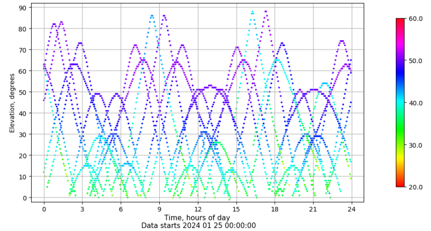
Time-elevation plot for station TAR0. Signal to Noise S1C Data file TAR000ESP_R_2024025.xtr
