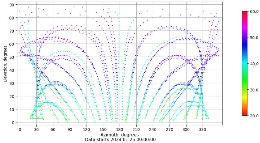
Azimuth-elevation plot for station TAR0. Signal to Noise S1C Data file TAR000ESP_R_2024025.xtr
