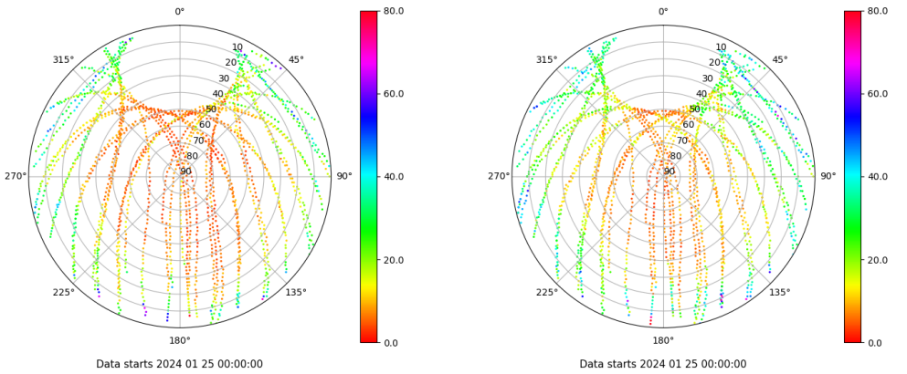
Skyplot for station TAR0. Parameter M1C Data file TAR000ESP_R_2024025.xtr Skyplot for station TAR0. Parameter M2P Data file TAR000ESP_R_2024025.xtr
