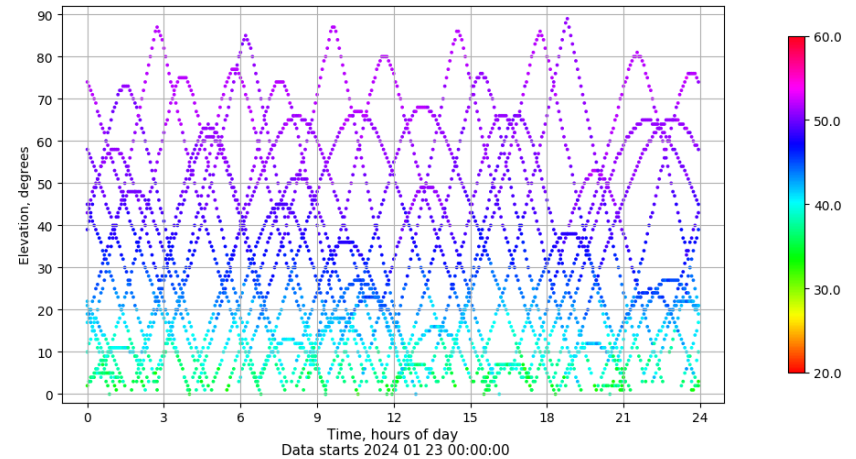
Time-elevation plot for station TAR0. Signal to Noise S1C Data file TAR000ESP_R_2024023.xtr
