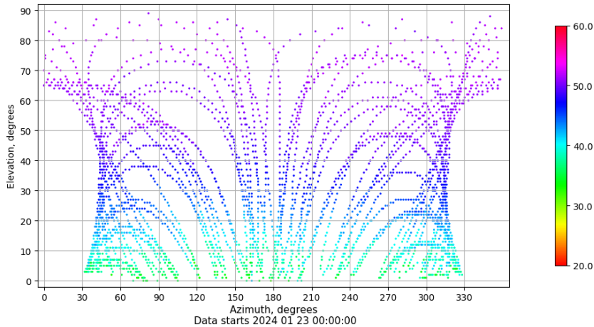
Azimuth-elevation plot for station TAR0. Signal to Noise S1C Data file TAR000ESP_R_2024023.xtr
