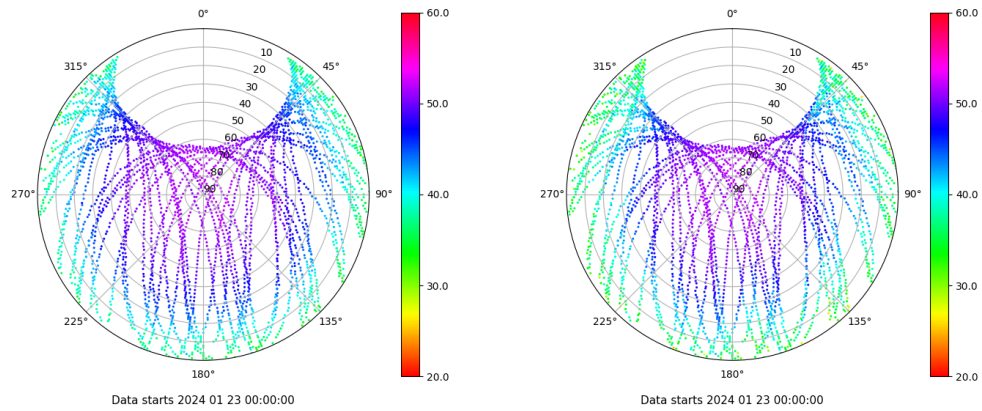
Skyplot for station TAR0. Signal to Noise S1C Data file TAR000ESP_R_2024023.xtr Skyplot for station TAR0. Signal to Noise S2W Data file TAR000ESP_R_2024023.xtr
