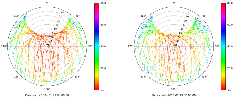
Skyplot for station TAR0. Parameter M1C Data file TAR000ESP_R_2024023.xtr Skyplot for station TAR0. Parameter M2W Data file TAR000ESP_R_2024023.xtr
