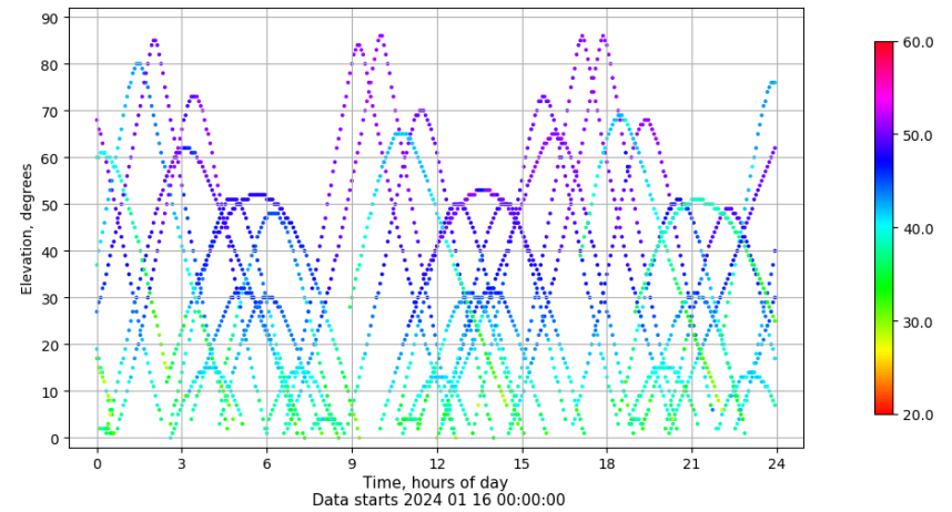
Time-elevation plot for station TAR0. Signal to Noise S1C Data file TAR000ESP_R_2024016.xtr
