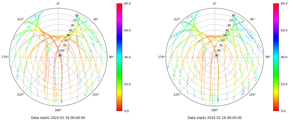
Skyplot for station TAR0. Parameter M1C Data file TAR000ESP_R_2024016.xtr Skyplot for station TAR0. Parameter M2P Data file TAR000ESP_R_2024016.xtr
