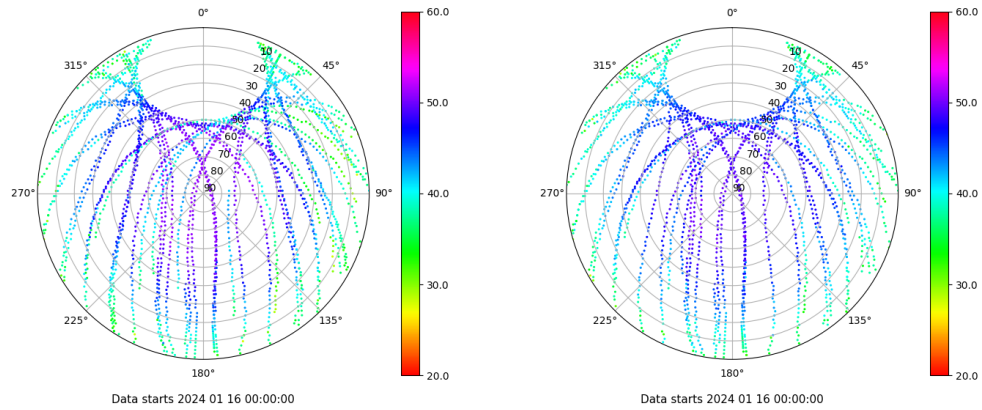
Skyplot for station TAR0. Signal to Noise S1C Data file TAR000ESP_R_2024016.xtr Skyplot for station TAR0. Signal to Noise S2P Data file TAR000ESP_R_2024016.xtr
