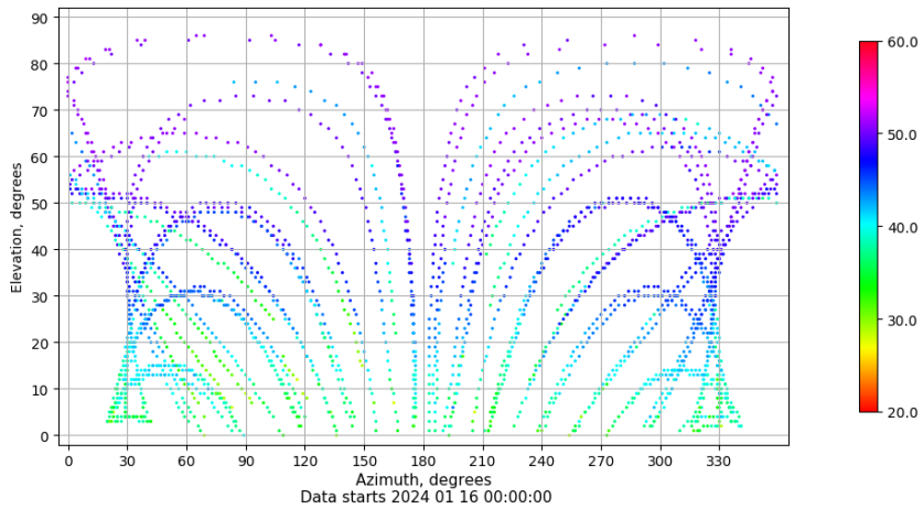
Azimuth-elevation plot for station TAR0. Signal to Noise S1C Data file TAR000ESP_R_2024016.xtr
