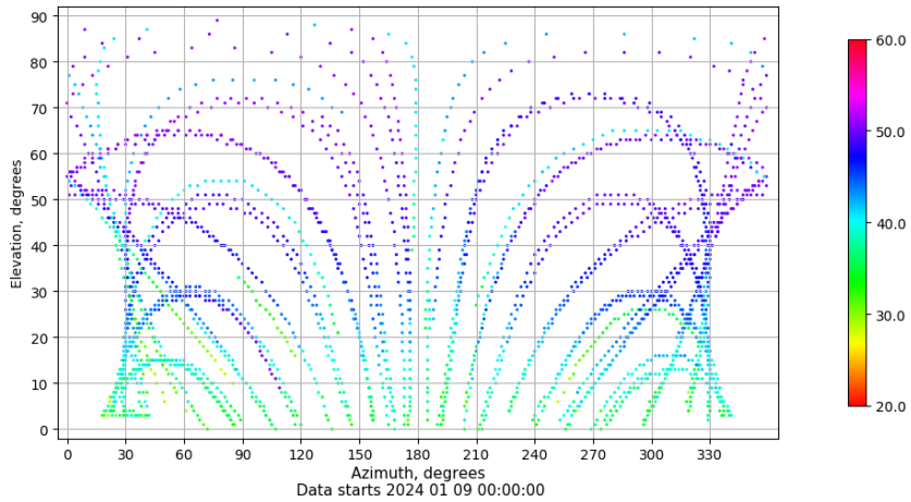
Azimuth-elevation plot for station TAR0. Signal to Noise S1C Data file TAR000ESP_R_2024009.xtr
