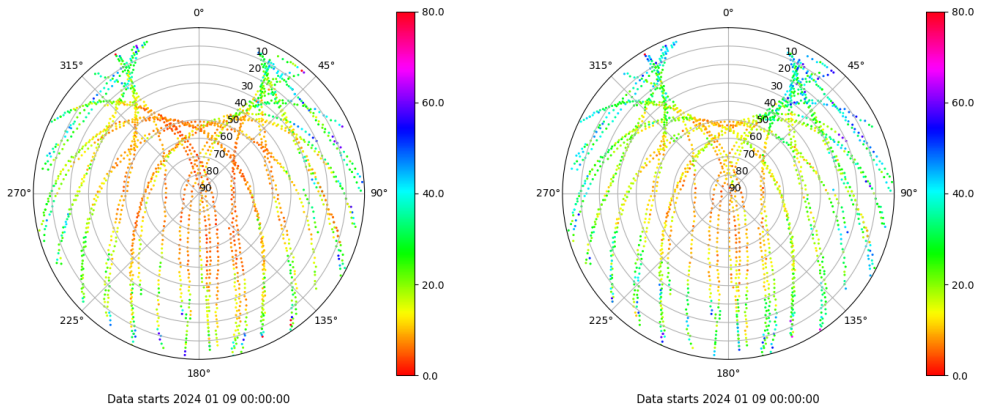
Skyplot for station TAR0. Parameter M1C Data file TAR000ESP_R_2024009.xtr Skyplot for station TAR0. Parameter M2P Data file TAR000ESP_R_2024009.xtr
