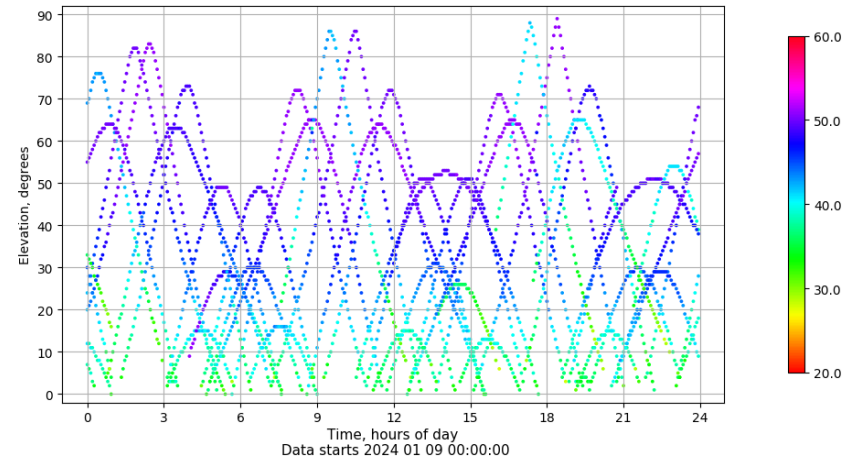
Time-elevation plot for station TAR0. Signal to Noise S1C Data file TAR000ESP_R_2024009.xtr
