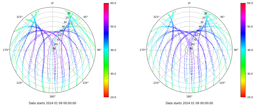
Skyplot for station TAR0. Signal to Noise S1C Data file TAR000ESP_R_2024009.xtr Skyplot for station TAR0. Signal to Noise S2P Data file TAR000ESP_R_2024009.xtr
